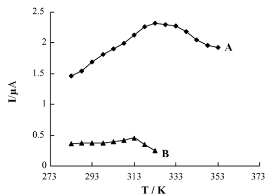
Fig. 4. Relationship between temperature value and response current of the uricase/ZnS QDs/L-cys/Au (A) and uricase/L-cys/Au (B) in PBS containing 5.0 \times 10^{-4} mol L ^{-1} uric acid.
