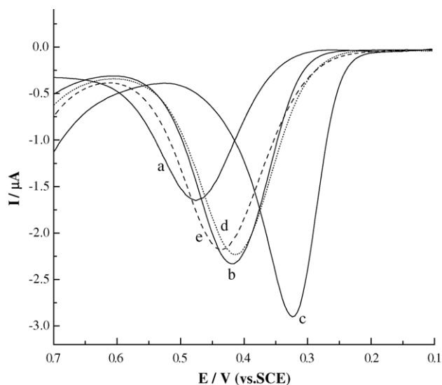
Fig. 3. The effect of pH on the uricase/ZnS QDs/L-cys/Au in PBS containing 5.0 \times 10^{-4} mol L ^{-1} uric acid: (a) pH 5.0; (b) pH 6.0; (c) pH 6.9; (d) pH 8.0; (e) pH 9.0.
