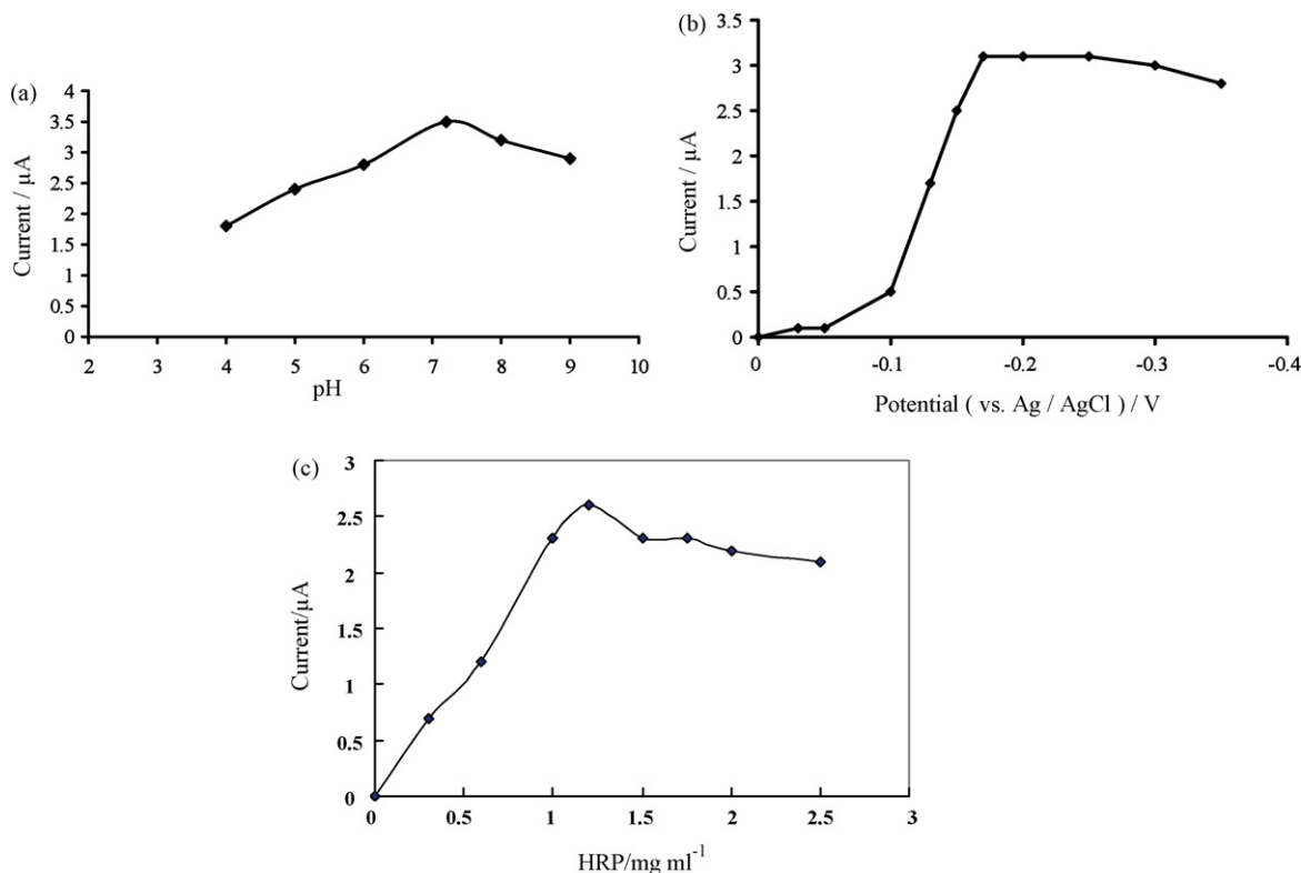
Fig. 6. (a) Influence of pH on the H_2O_2 sensor, study-state current measured in the presence of 0.5 mM H_2O_2 in 0.1 M PBS (pH 7.2) at applied potential of -0.18 at 25^\circ\text{C} . (b) Effect of potential on the sensor response for 0.5 mM H_2O_2 in 0.1 M PBS (pH 7.2). (c) Influence of the amount of HRP on the fabrication of biosensor.
