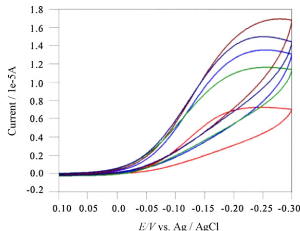
Fig. 5. Cyclic voltammograms of MWCNTs/MG/HRP/GCE in the presence of different concentration of H_2O_2 : 0.3 0.5, 0.7, 1.0, 1.2 mM in 0.1 M PBS (pH 7.2) at the scan rate of 50 \text{ mV s}^{-1} .
