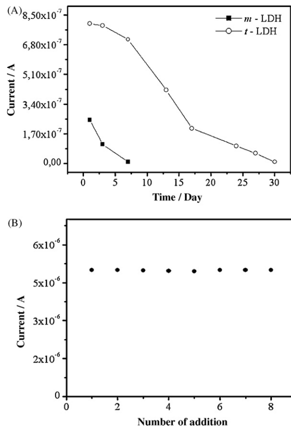
Fig. 6. (A) Stability of working electrodes t -LDHE and m -LDHE (B) Stability of thermostable lactate biosensor using the t -LDHE for sequential measuring at lactate concentration of 10 mM.
