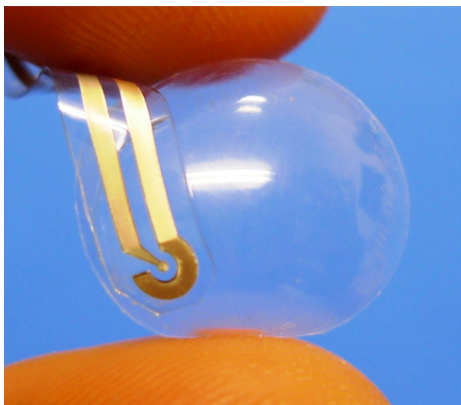
Fig. 3. Photograph of the CL biosensor constructed by biocompatible materials (PDMS and hydrophilic PME) and the flexible electrodes (Pt working and Ag/AgCl counter/reference film electrodes formed onto the PMDS membrane).
