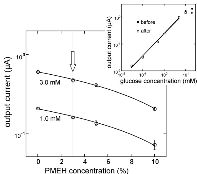
Fig. 6. Output current variation caused by a coating concentration of PME (no PME, 3%, 5%, 10%) 1.0 and 3.0 mM glucose. The largest current was shown in case of no PME-coating. The current decreased with the increasing of PME concentration. Inset box is calibration curves of the biosensor before and after application. (●) Before application; (□) after application.
