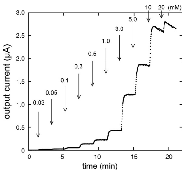
Fig. 4. Typical response of the CL biosensor with no PME-coating to glucose concentration in vitro (constant voltage of +400 mV vs. Ag/AgCl, pH 7.4, 20 mM phosphate buffer solution). The output current increased immediately after the glucose solution was dropped into PBS.
