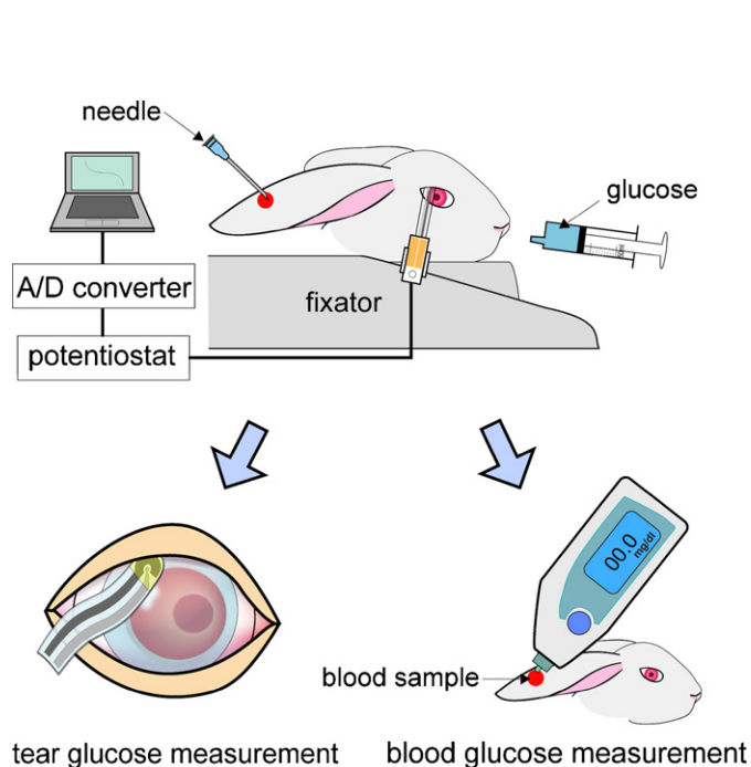
Fig. 2. Measurement method of tear glucose concentration with the CL biosensor. Blood glucose level was measured by a commercially blood glucose monitoring kit, simultaneously.
