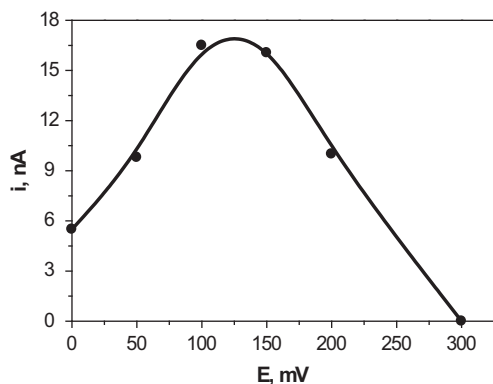
Fig. 1. Effect of applied potential on the amperometric signal measured for 1.0 \times 10^{-4} \text{ mol L}^{-1} sucrose in a 0.05 \text{ mol L}^{-1} phosphate buffer solution (pH 6.0) at the INV/FDH biosensor.
