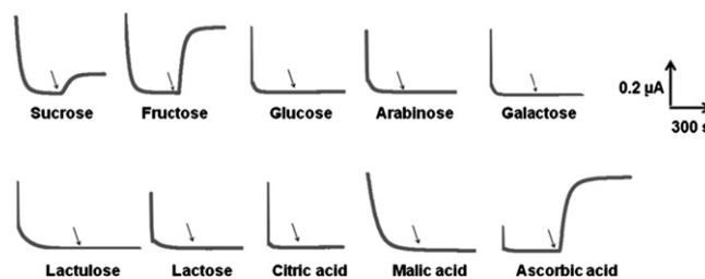
Fig. 2. Amperometric responses obtained at the INV–TTF–FDH–AuE biosensor upon 50 \mu\text{L} additions of 0.1 \text{ mol L}^{-1} solutions of different interfering compounds to 0.05 \text{ mol L}^{-1} phosphate buffer (pH 6.0). E_{\text{app}} = +0.10 \text{ V} (vs Ag/AgCl).
