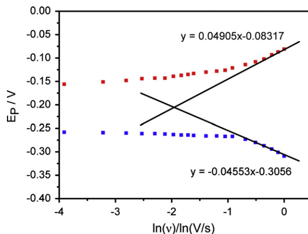
Fig. 7. Relationship between the peak potential ( E_p ) and the natural logarithm of scan rate for MP-11/MBA-Au-cavities/ITO electrode in pH 7.0 PBS.
