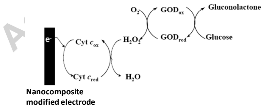
Scheme 1. The reaction illustration of the GOD/Cyt c /GNPs/PANS/GC bienzyme electrode.
