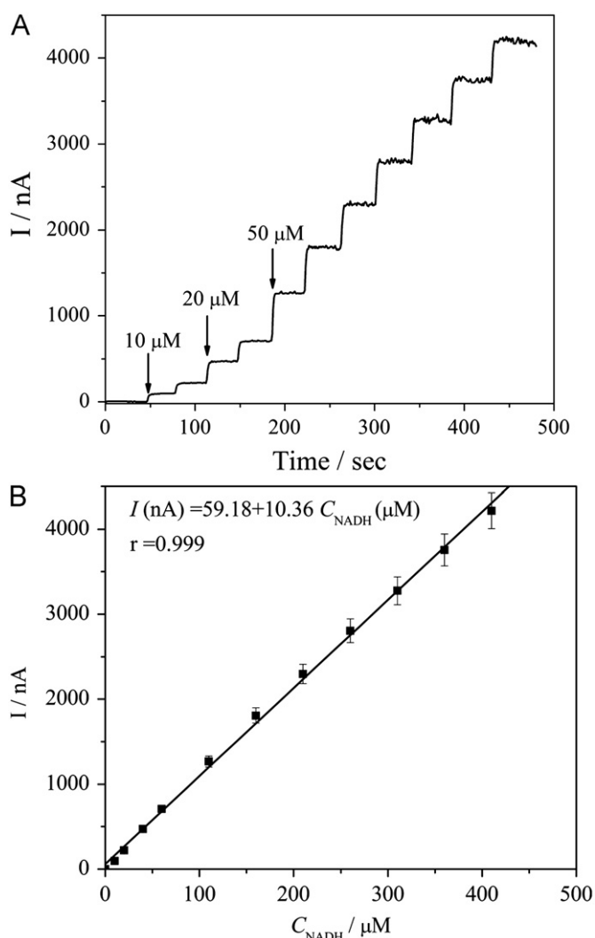
Fig. 4. (A) Amperometric responses of the MDB/GMCs/CS/SPE upon successive addition of NADH ( 10 , 20 and 50 \mu\text{M} ) in a stirred Tris-HCl buffer solution (0.1 M, pH 8.0, 300 rpm) and (B) the corresponding calibration curve of the response currents and the concentrations of NADH. Working potential: -0.15 \text{ V} . The error bars indicate 95% confidence interval of steady-state currents.
