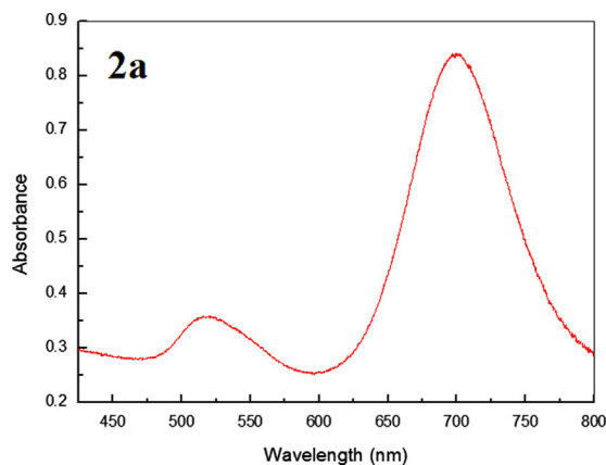
Fig. 2. UV–vis absorption spectra (a) and TEM images (b) of GNRs.
