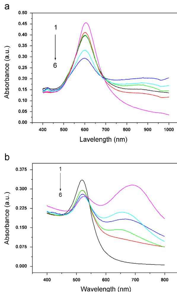
Fig. 2. Absorption spectra of Au–Ag–Au double shell nanoparticles (a) and gold nanosphere (b) in the presence of different methimazole concentrations. Concentrations of methimazole from (1 to 6) 0.0, 0.1, 0.3, 0.5, 1.0 and 3.0 \times 10^{-7} \text{ mol L}^{-1} and (b) 0.0, 0.5, 1, 2, 3 and 5.0 \times 10^{-7} \text{ mol L}^{-1} .
