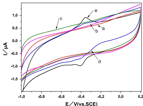
Fig. 7. Cyclic voltammograms of different modified electrodes in 0.1 M PBS (pH=7.0) containing 0.1 M KCl. Bare GCE electrode (a); the ( \text{SiO}_2 NPs)/GCE electrode (b); the ( \text{SiO}_2\text{-P} NPs)/GCE electrode (c); the XOD/( \text{SiO}_2 NPs)/GCE electrode (d) and the XOD/( \text{SiO}_2\text{-P} NPs)/GCE electrode (e) (scan rate is 100 \text{ mV s}^{-1} ).
