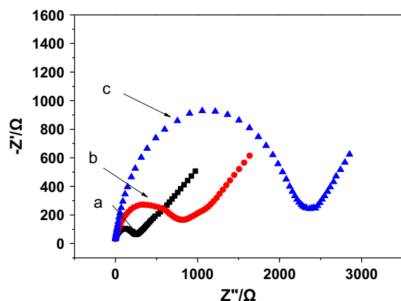
Fig. 6. EIS in 0.1 mM KCl containing 0.5 mM \text{K}_3\text{Fe}(\text{CN})_6/\text{K}_4\text{Fe}(\text{CN})_6 , (a) bare, (b) \text{SiO}_2\text{-P} modified and (c) \text{SiO}_2 modified GCE electrode.
