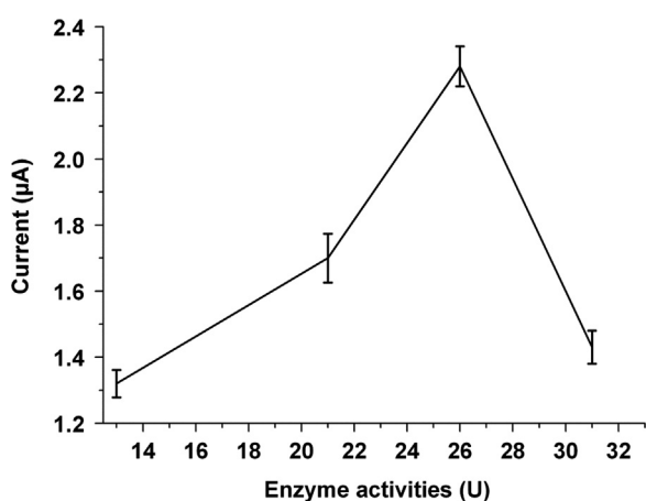
Fig. 4. Effect of loaded enzyme amount (in phosphate buffer, 50 mM, pH 7.0, 25 °C). The corresponding measurements were performed with 25 \mu M cholesterol. Error bars show standard deviation (SD) of four measurements.
