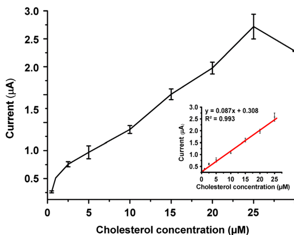
Fig. 7. Calibration curve for cholesterol (in 50 mM phosphate buffer, pH 7.0, 25 °C). Error bars show standard deviation (SD) of four measurements.
