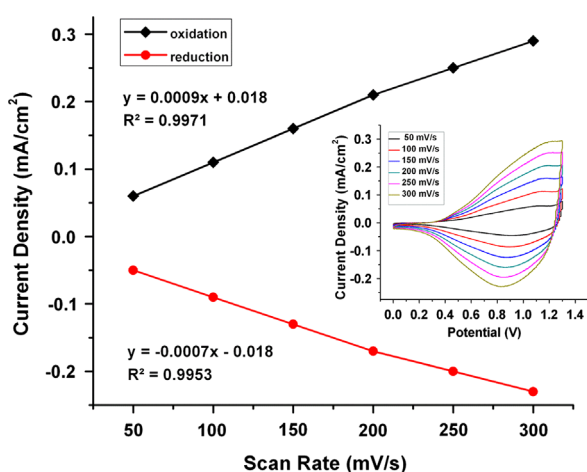
Fig. 3. Scan rate dependence of poly (BIPF) film in 0.1 M NaClO 4 –LiClO 4 /DCM/ACN at 50, 100, 150, 200, 250 and 300 mV s −1 .
