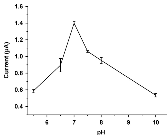
Fig. 5. Effect of pH (50 mM sodium phosphate buffer at pH 5.5; 6.5, 7.0; 7.5 and 50 mM sodium bicarbonate buffer at pH 8.0 and 10.0, 25 °C). The corresponding measurements were performed with 25 \mu M cholesterol. Error bars show standard deviation (SD) of four measurements.
