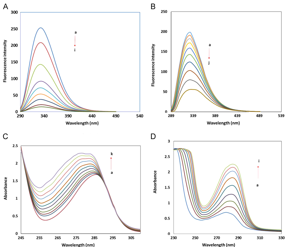
Fig. 5. (A) Fluorescence emission spectra of the BSA-MWCNTs system in PBS (0.067 M, pH 7.4) at 298.15 K: (a) free BSA (20.0 μM), and (b–i) BSA 20.0 μM with MWCNTs at 5.0, 10.0, 20.0, 30.0, 40.0, 50.0, 60.0, and 80.0 μM, (B) fluorescence emission spectra of the BSA-BN system in PBS (0.067 M, pH 7.4) at 298.15 K: (a) free BSA (15.0 μM), and (b–j) BSA 15.0 μM with BN at 2.0, 4.0, 5.0, 10.0, 20.0, 30.0, 40.0, 50.0, and 60.0 μM, (C) UV-vis absorption spectra of the BSA-MWCNTs system in PBS (0.067 M, pH 7.4): (a) free BSA (1.0 μM), and (b–k) BSA 1.0 μM with MWCNTs at 0.1, 0.2, 0.3, 0.4, 0.5, 0.6, 0.7, 0.8, 0.9, and 1.0 μM, and (D) UV-vis absorption spectra of the BSA-BN system in PBS (0.067 M, pH 7.4): (a) free BSA (1.0 μM), and (b–i) BSA 0.5 μM with BN at 0.5, 1.0, 1.5, 2.0, 2.5, 3.0, 3.5, and 4.0 μM.
