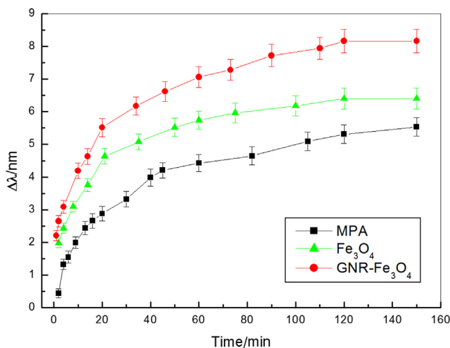
Fig. 6. Kinetic adsorption curves of immobilizing goat anti-mouse IgG at the concentration of 75 \mu\text{g mL}^{-1} on SPR biosensors based on MPA, Fe 3 O 4 nanoparticles and GNR-Fe 3 O 4 nanohybrids.
