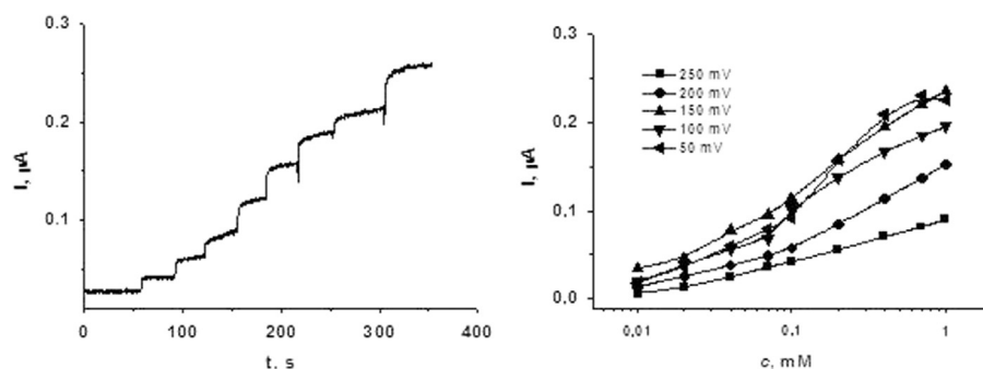
Fig. 3. Dynamic response of AChE sensor with CB, Ag nanoparticles and AChE (6.25 U/mL, aliquot 2 μL) on 20, 60 μM, 0.1, 0.2, 0.4, 1.0 and 2.0 mM ATCh at 150 mV and dependence of the signal on the working potential. Chronoamperometric regime, PBS, pH 7.8.
