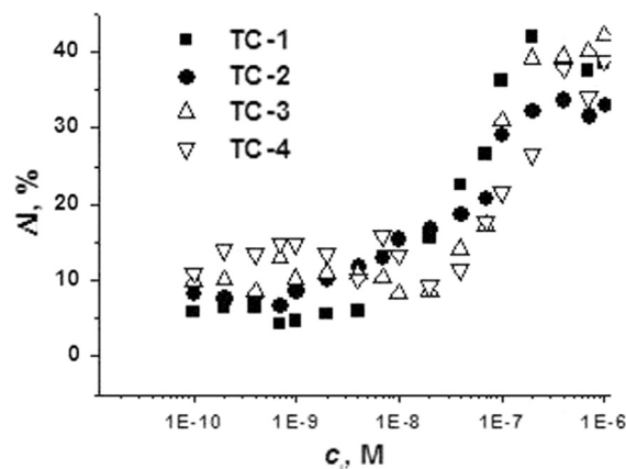
Fig. 6. Calibration plots of malaoxon obtained with AChE sensor based on glassy carbon modified with CB and Ag nanoparticles in the presence of 1.0 \mu M protecting agents TC-1, TC-2, TC-3, TC-4. Incubation 10 min, PBS, pH=7.8.
