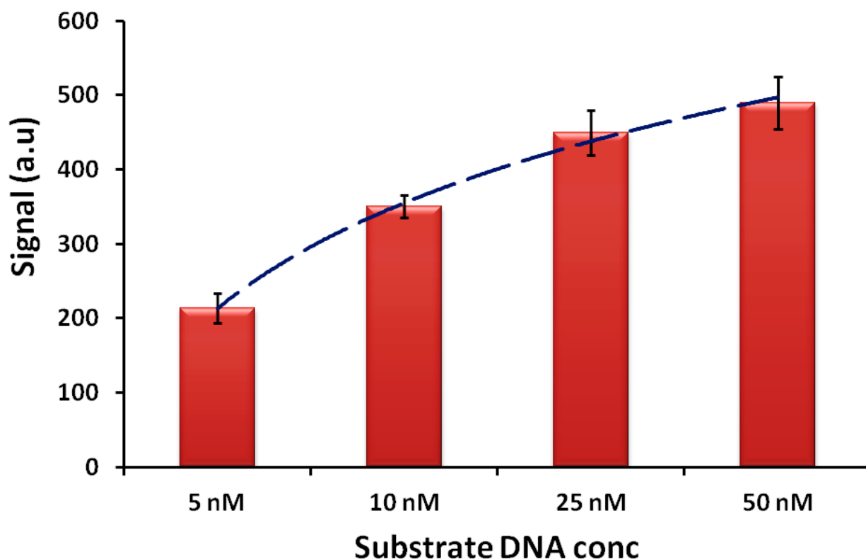
3 Figure 4 Experimental optimization of the fluorescent-labeled substrate DNA concentration for 4 pre-mixing step. \Delta S is the fluorescent intensity difference between peak intensity and base-line. 5 Each data value is the average of two independent experimental results.
