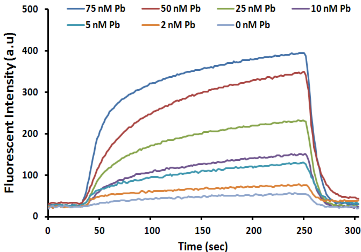
Figure 7 The fluorescence intensity responses during a typical test cycle for different amount of lead (II) ion using the optical sensor system, including the BSA treatment for blocking non-specific sites.
