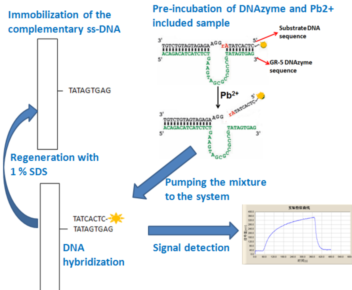
Figure 1 Schematic representation of sensing mechanism for Lead (II) ion detection using a optical fiber sensing platform and employing DNAzyme as a recognition agent. The sensing mechanism starts with pre-incubation step (enzymatic reaction) and continues with hybridization of product of the substrate DNA and probe-DNA, signal detection and regeneration steps.
