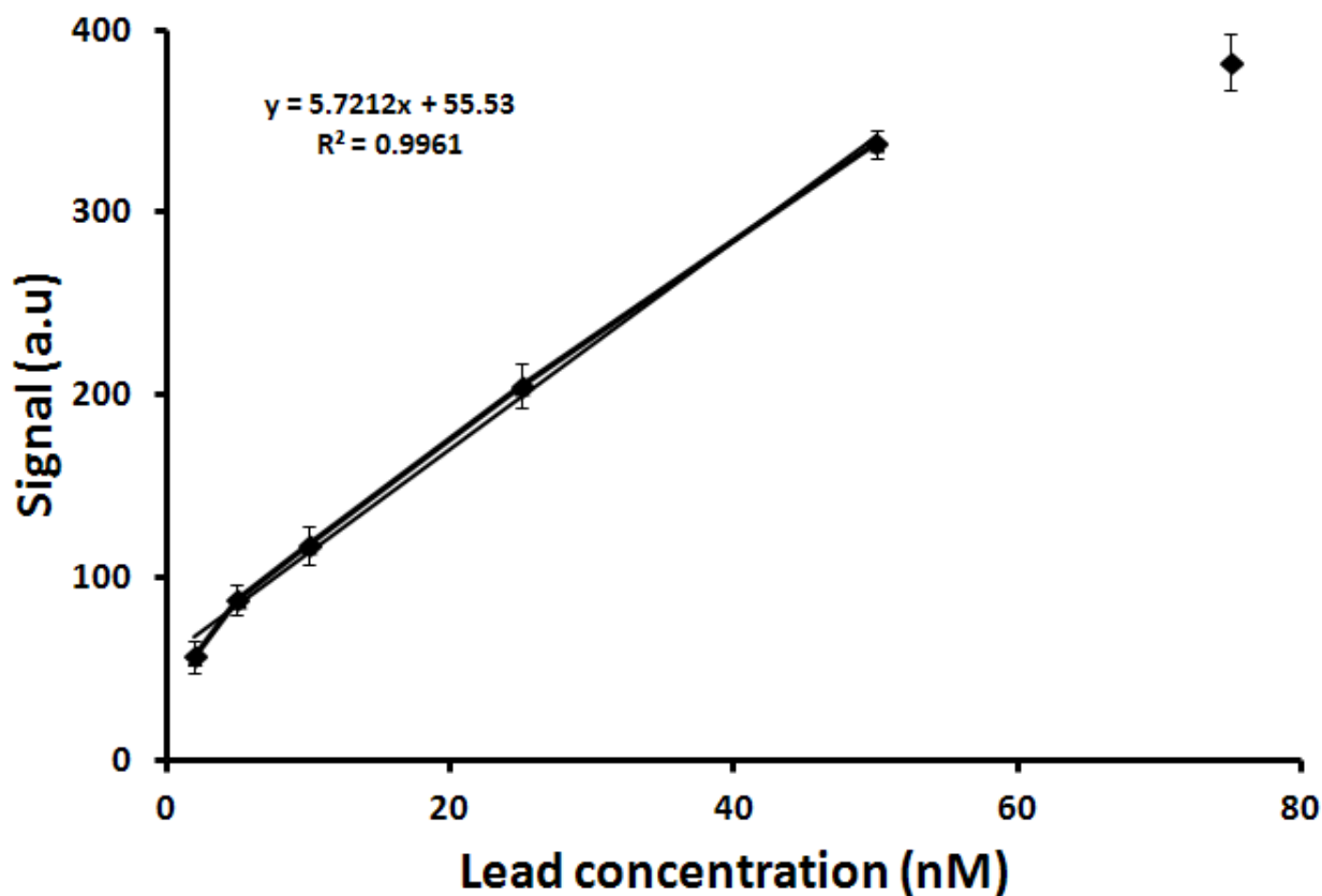
Figure 8 The calibration plot for determination of lead (II) ion concentration using the DNAzyme based fiber optic biosensor system. Signal is the fluorescent intensity difference between peak intensity and base-line. Each data value is the average of three independent experimental results.
