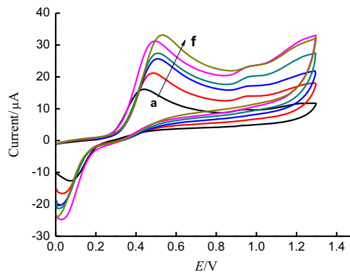
Fig. 11. The CV of dsDNA/PANI/CTS/GCE electrode in acetic acid buffer with 7.5 \times 10^{-5} M hydroquinone with different sweep speed. (a) 20 \text{ mV s}^{-1} , (b) 40 \text{ mV s}^{-1} , (c) 60 \text{ mV s}^{-1} , (d) 80 \text{ mV s}^{-1} , (e) 100 \text{ mV s}^{-1} , and (f) 120 \text{ mV s}^{-1} .
