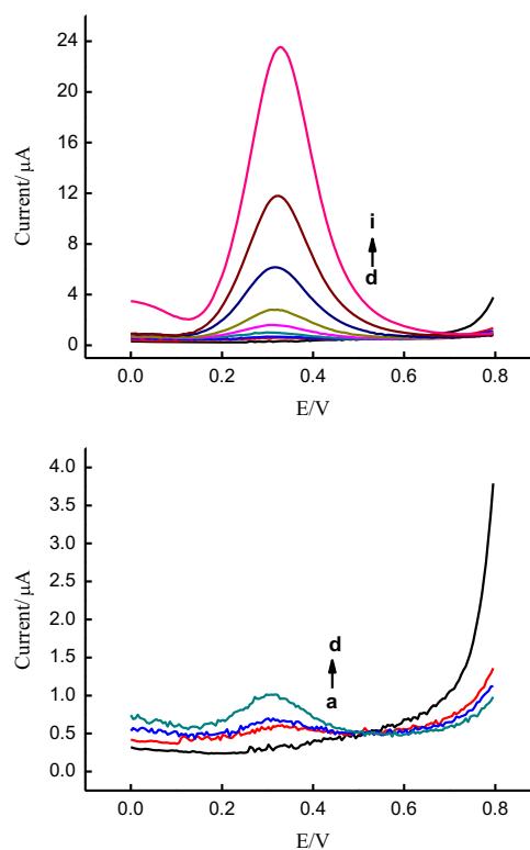
Fig. 6. The responses of the dsDNA/PANI/CTS/GCE electrode in 0.2 M HAc buffer (pH=4.4) with different concentrations of hydroquinone. (a) 1.25 \times 10^{-6} M, (b) 2.5 \times 10^{-6} M, (c) 5.0 \times 10^{-6} M, (d) 1.0 \times 10^{-5} M, (e) 2.0 \times 10^{-5} M, (f) 4.0 \times 10^{-5} M, (g) 8.0 \times 10^{-5} M, (h) 1.6 \times 10^{-4} M and (i) 3.2 \times 10^{-4} M.
