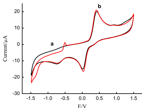
Fig. 9. The influence of \text{Na}^+ on CV of the dsDNA/PANI/CTS/GCE interact with 7.5 \times 10^{-4} M hydroquinone in HAc buffer. (a) without NaCl and (b) with 0.03 M NaCl.
