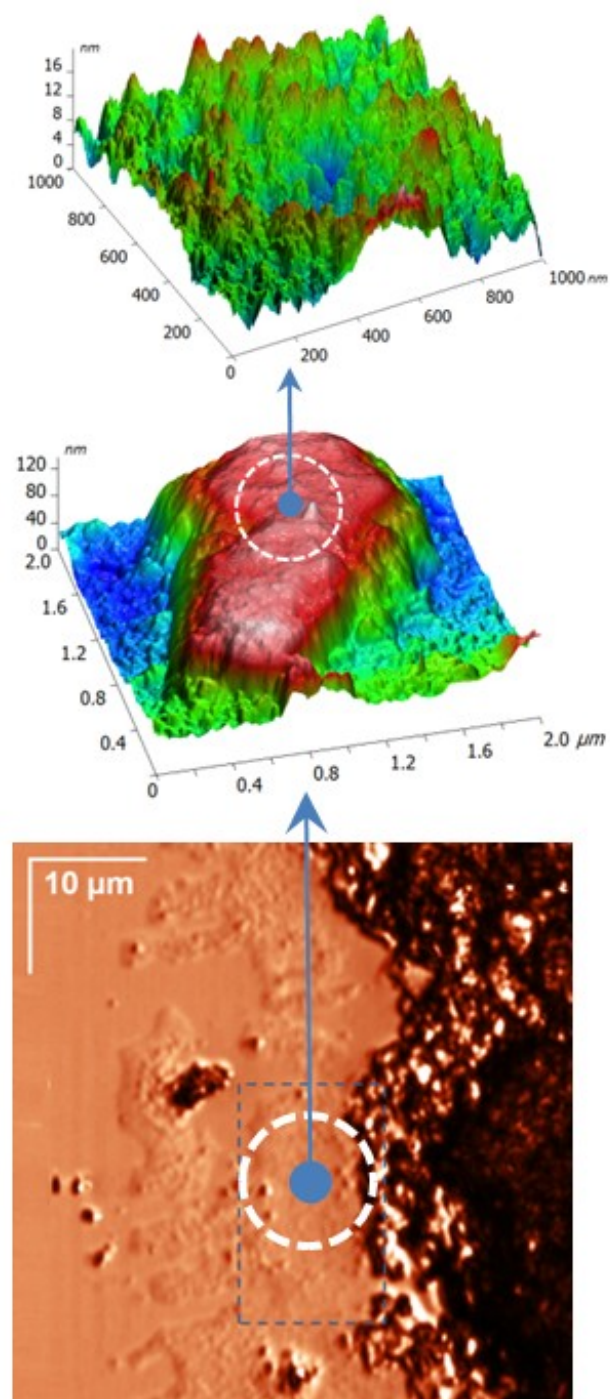
Fig.2 Optical image (bottom) of dried yeast envelope solution containing both single and multilayer areas as well as AFM images of single cell envelope (middle) and topography of membrane surface (top). Thickness of single layer area is above 100-120 nm.
