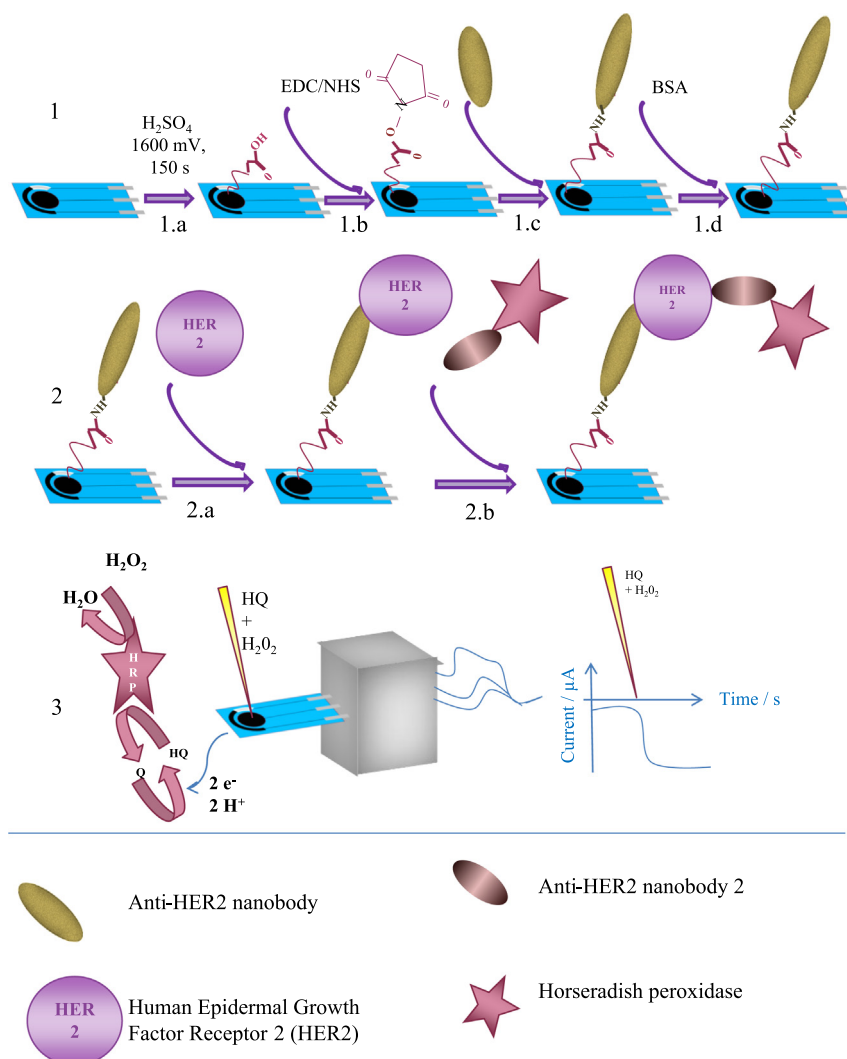
Fig. 1. Schematic drawing of SPE modification. (1) and nanoimmunoassay (2 and 3). 1. SPE oxidation to generate carboxylic groups (1a), activation of the carboxylic groups with EDC and NHS (1b), immobilization of the anti-HER2 Nb (1c), blocking of the free sites by BSA (1d); 2. Sandwich nanoimmunoassay: HER2 sample incubation (2a), Nb-HRP incubation (2b); 3. Amperometric detection of p-quinone (Q) generated by HRP in the presence of HQ and \text{H}_2\text{O}_2 .
