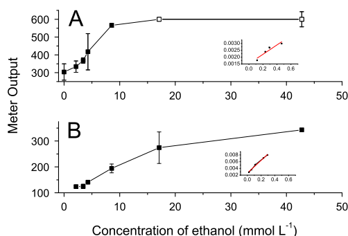
Fig. 4. Glucose meter response to a mixture of ethanol and detection reagent solution (1:1 v/v ratio), applied to \mu PEDs. Meter response after (A) 3 insertions ( \sim 25 s) and (B) 5 insertions. Symbol \square denotes outputs that included “HI.” Lineweaver-Burke Plots are shown in the corresponding insets, R^2=0.8529 and 0.989 for (A) and (B), respectively. N=3 .
