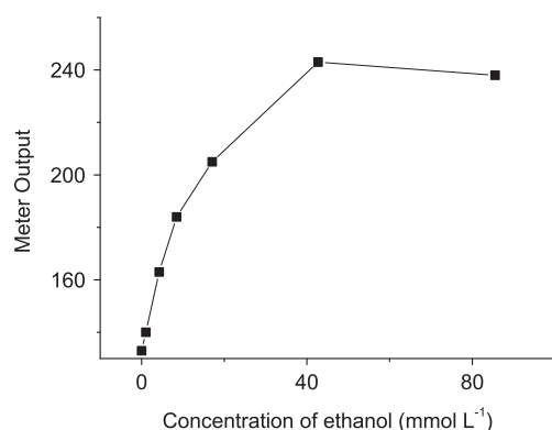
Fig. 7. Representative ethanol response using \mu PEDs and a glucometer with trehalose included in the detection reagent. Detection reagents were dried for 48 h at 4 °C. Results recorded after 6 insertions. Linear range between 2 mmol L -1 and 8 mmol L -1 had R^2=0.9482 .
