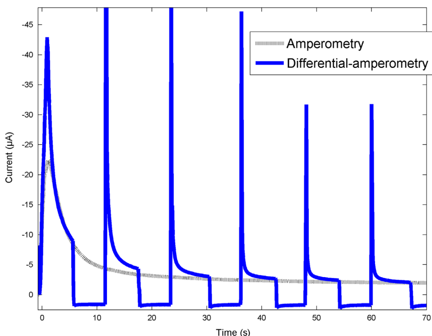
Fig. 3. Representative amperometric response to 8 mmol L -1 ethanol using a potentiostat and \mu PEDs. +0.4 V vs carbon was applied continuously (—) or cycled between +0.4 V and +0 V vs carbon every 5 s.
