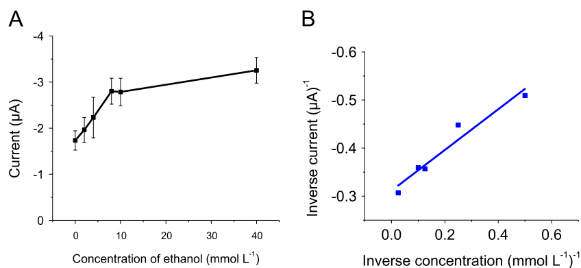
Fig. 6. Ethanol measurements using \mu PEDs and a potentiostat. (A) Current response and (B) Lineweaver-Burke Plot ( R^2=0.9449 ). Ethanol samples and detection reagents (1 mg/ml ADH, 15 mmol L -1 NAD + in 0.1 M PB) were mixed and applied directly to the \mu PED with a potential of +0.3 V vs C ( t=70 s). Results reported as the mean \pm 1 STD, n=4 .
