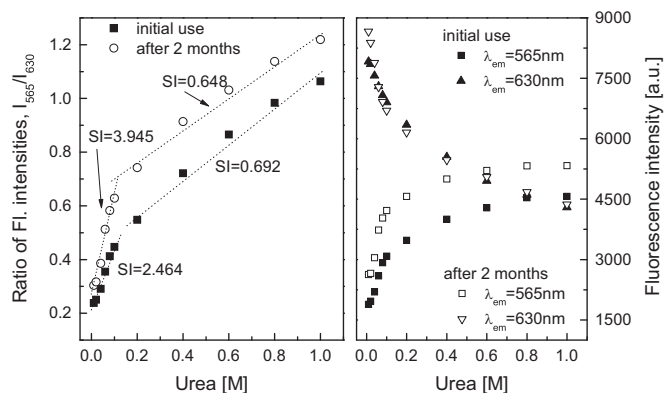
Fig. 8. Long-term stability of the urea-sensing membrane in the urea concentration range of 0.01 M to 1.0 M at initial use and after 2 months of use (left), and two emission fluorescence intensities at \lambda_{em}=565 nm and \lambda_{em}=630 nm (right).
