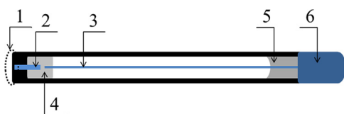
Fig. 1. Scheme of the platinum disc electrodes. 1—bioselective membrane, 2—platinum wire, 3—internal conductor, 4—Wood alloy, 5—epoxy resin, 6—contact pad.
