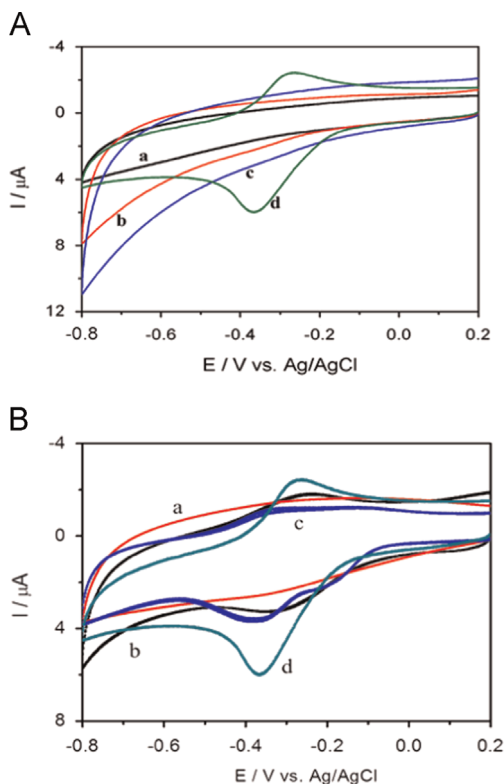
Fig. 3. A: The CVs of MP11/GCE (a), PDDA-G/GCE (b), DMPG-AuNPs/PDDA-G/GCE (c) and MP11/DMPG-AuNPs/PDDA-G/GCE (d) in N_2 -saturated PBS (0.1 M, pH 7.0) at the scan rate of 100 mV/s. B: The CVs of MP11/DMPG-AuNPs/GCE (a), MP11/PDDA-G/GCE (b), hemin/DMPG-AuNPs/PDDA-G/GCE (c) and MP11/DMPG-AuNPs/PDDA-G/GCE (d) in N_2 -saturated PBS (0.1 M, pH 7.0); scan rate: 100 mV s -1 .
