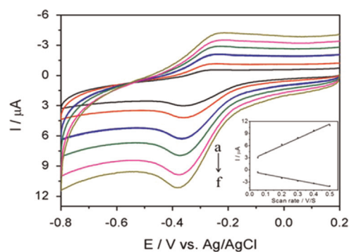
Fig. 4. The CV of MP11/DMPG-AuNPs/PDDA-G/GCE at scan rates of 50, (a) 100, (b) 200, (c) 300, (d) 400, (e) 500 mV/s, and (f) in N_2 -saturated PBS (0.1 M, pH 7.0). Inset: the linear dependence of peak currents on scan rate.
