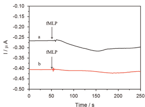
Fig. 6. The responses of the biosensor in N_2 -saturated PBS (0.1 M, pH 7.0) with the addition of fMLP at 50 s, with MCF-7 cells (a) and without MCF-7 cells (b).
