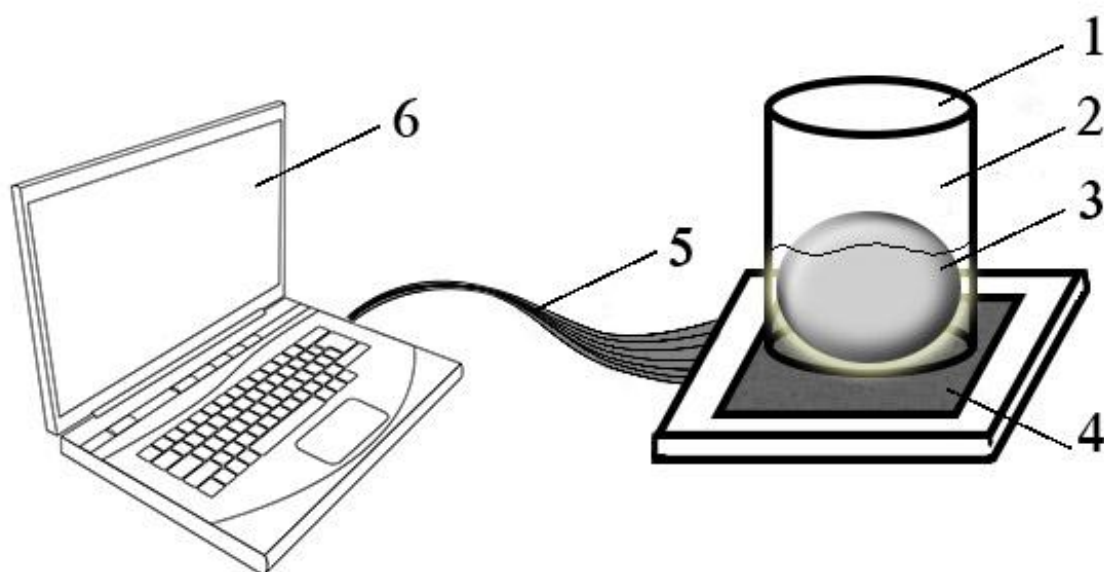
Figure1: Schematic presentation of the biosensor. where 1 is a flat bottom insert 2. A liquid sample 3. A bioreporter pad 4.A CMOS photodetector 5. A USB cable 6. A laptop
