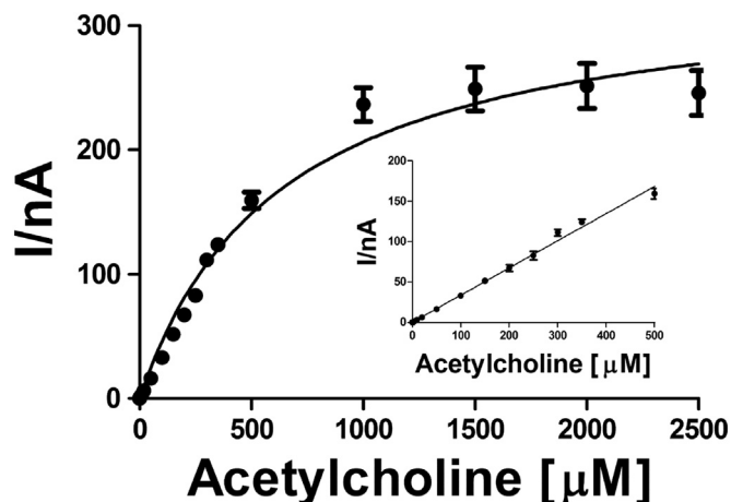
Fig. 4. In vitro calibration of a Cox/ACE biosensor, incorporating a p-magnolol permeselective film, showing Michaelis-Menten kinetics and linear regression (inset); n=4 .
