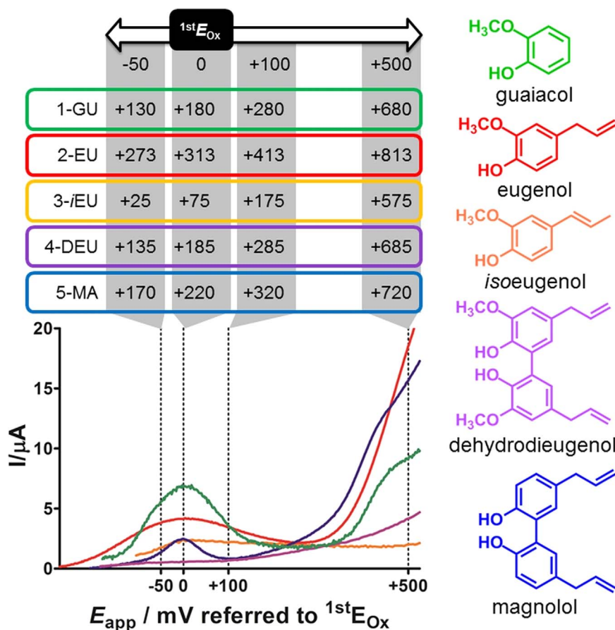
Fig. 1. First oxidation peak potentials ( 1^{\text{st}} E_{\text{Ox}} ) and potential referred to Ag/AgCl reference electrode are reported in the table. The graphic shows the CV first cycle of each phenol setting the 1^{\text{st}} E_{\text{Ox}} as 0, only the forward part is reported. Structures of studied phenols are on the right.
