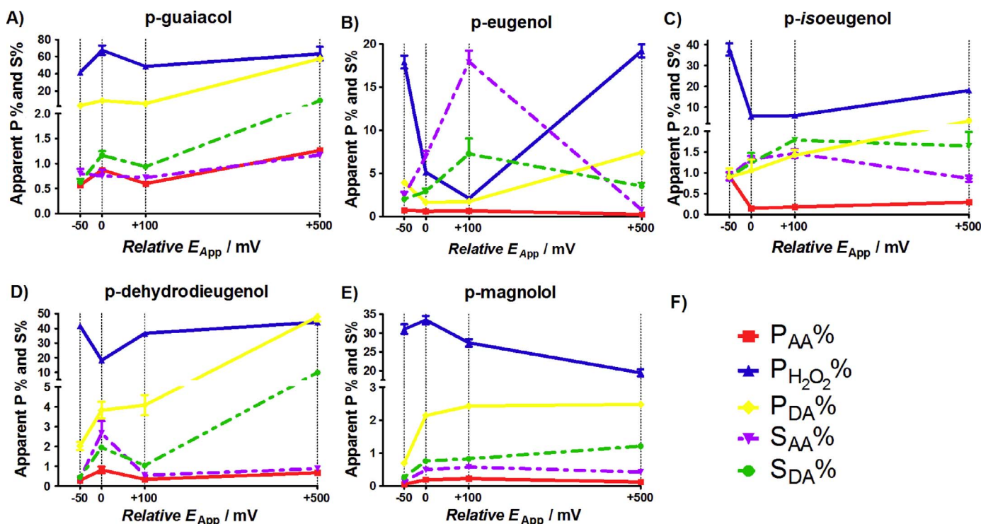
Fig. 2. Selectivities (S%) and apparent permeabilities (P%) of phenol-derived polymeric film versus relative polymerization potential (relative E_{app} ) at day 1; n=4 .
