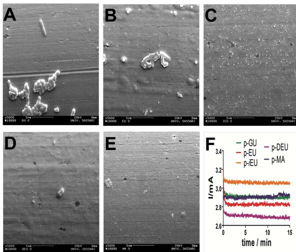
Fig. 3. SEM microphotographs at 5000 \times magnification of phenol polymerized at a relative E_{\text{app}} of 0 mV. A: p-guaiacol (p-GU); B: p-eugenol (p-EU); C: p-isoeugenol (p-iEU); D: p-dehydrodieugenol (p-DEU); E: p-magnolol (p-MA); F: time course of polymerizations of phenols at relative E_{\text{app}} of 0 mV.
