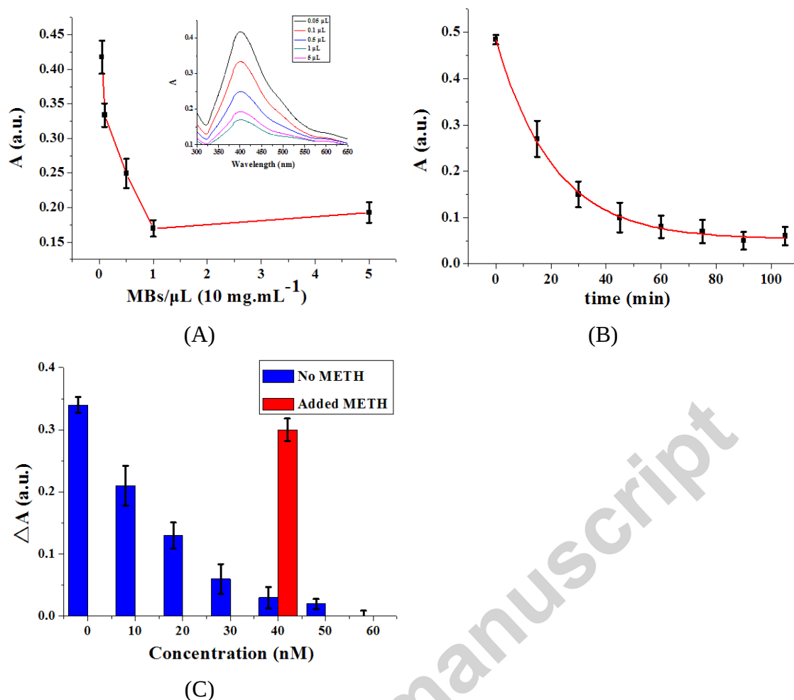
Fig 2. (A) SPR signal intensities at different MBs concentrations. The curve and UV-vis spectra (insert) of the supernatant at different concentrations of MBs. Under the same concentration of METH aptamer (40 nM), the sensitivity of assay positively correlated with variation of SPR peak intensity. (B) Hybridization reaction time of SPR signal intensity change at 400 nm with METH aptamer concentration of 40 nM. (C) SPR signal intensities of the Au@Ag ( \lambda_{\text{max}}=400 \text{ nm} ) in the presence of different concentrations of METH aptamer (Blue). Red bar is SPR signal intensity of the Au@Ag in the presence of METH (100 nM). The signal ( \Delta A ) is expressed as the relative absorbance with respect to the blank and error bars represent three replicate measurements (same for below).
