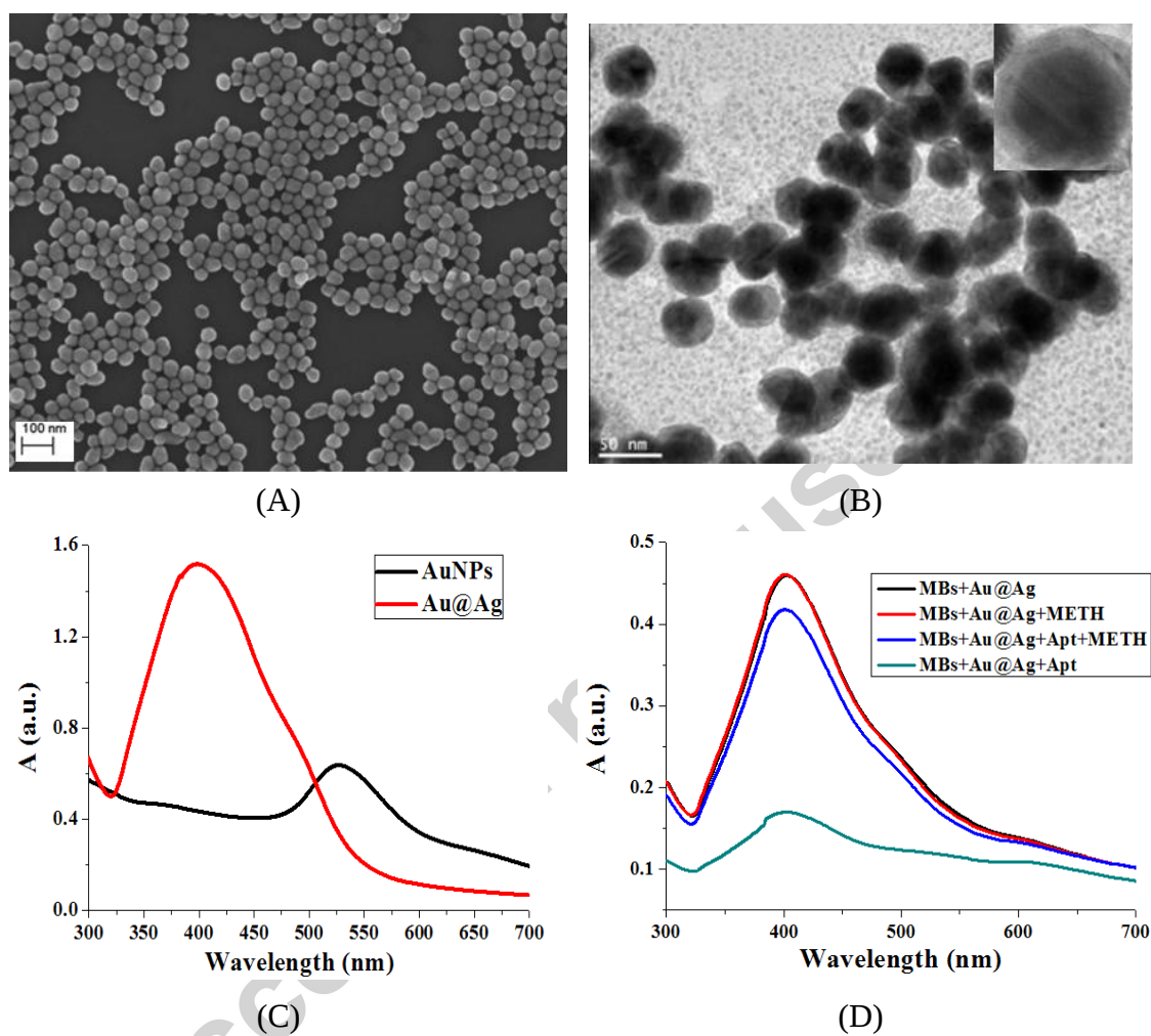
Fig 1. (A) Scanning electron microscope (SEM) image and (B) high resolution transmission emission microscope (HR-TEM) image of prepared Au@Ag core-shell nanoparticles. (C) SPR signal of Au@Ag and AuNPs. (D) UV-vis spectra of Au@Ag in the presence or absence of METH. The signal (A) is the absorbance of Au@Ag core-shell nanoparticles and error bars represent triplicate measurements (same for below).
