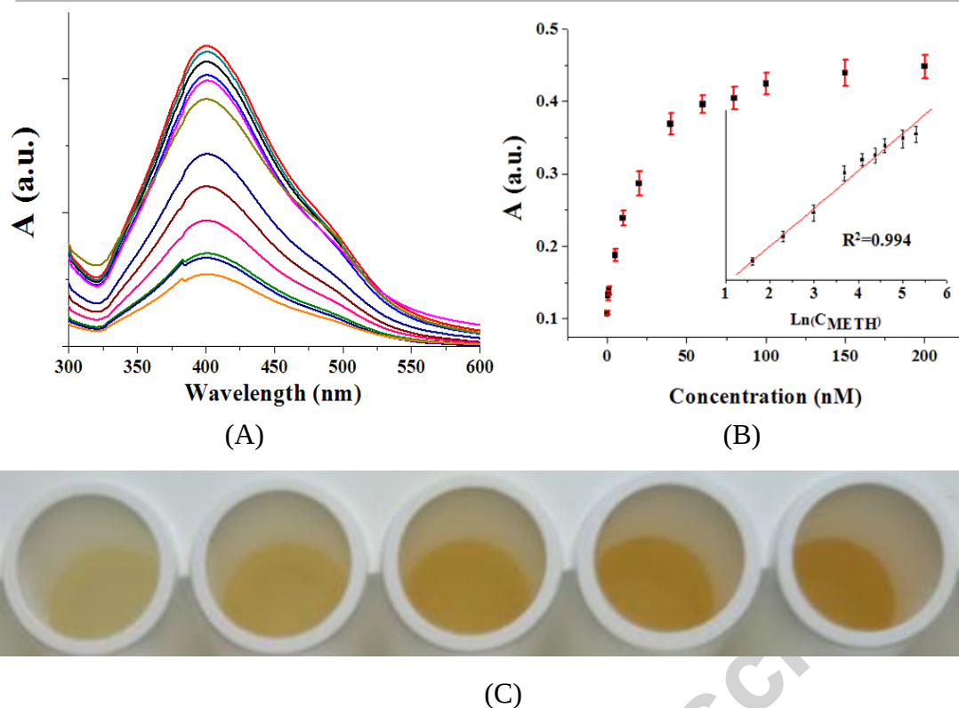
Fig 3. (A) UV-vis spectra of Au@Ag in the presence of different concentrations of METH (from bottom to up: 0, 0.5, 1, 5, 10, 20, 40, 60, 80, 100, 150, 200 nM). (B) SPR signal intensity ( \lambda_{\max}=400 nm) at various METH concentrations (The inset shows the logarithm linear range concentration (0.5-200.0 nM)). (C) Color change of the non-aggravation Au@Ag in the presence of METH. The METH concentrations in tubes from left to right were: 0, 5, 10, 50, and 100 nM.
