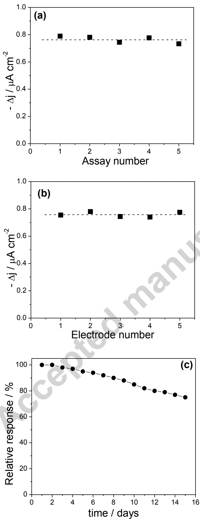
Figure 6. Graphical representation of (a) repeatability; (b) reproducibility and (c) stability of the XOD/GCE biosensor.
