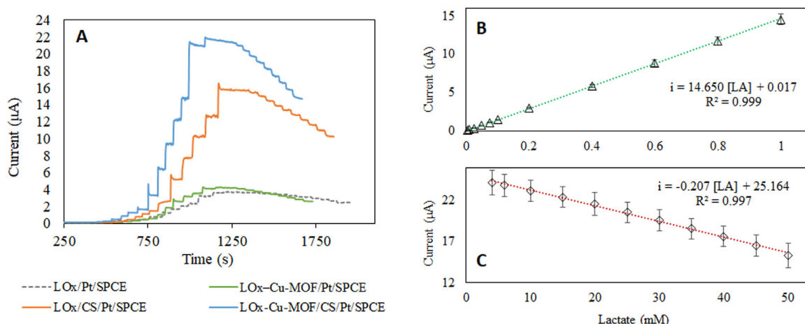
Fig. 1. A: Amperograms obtained at different LO x based biosensors in 5 mL of phosphate buffer pH 7.0, for successive additions of lactate ranging from 0.75 \mu M up to 50 mM. Eap: 0.15 V; (grey) LO x /Pt/SPCE; (green) LO x -Cu-MOF/Pt/SPCE; (orange) LO x /CS/Pt/SPCE, and (blue) LO x -Cu-MOF/CS/Pt/SPCE. Calibration curves in catalysis (B) and inhibition (C) zones obtained in optimal conditions, corresponding to amperogram (blue) LO x -Cu-MOF/CS/Pt/SPCE (For interpretation of the references to color in this figure legend, the reader is referred to the web version of this article.).
