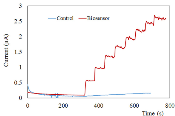
Fig. 3. Amperograms recorded at LO x -Cu-MOF/CS/Pt/SPCE (red curve) and at control Cu-MOF/CS/Pt/SPCE (blue curve), for the determination of lactate in wine samples. Successive additions of 10 µL of red wine in phosphate buffer (0.1 M, pH 7.0), at Eap: 0.15 V (vs SPE Ag/AgCl).
