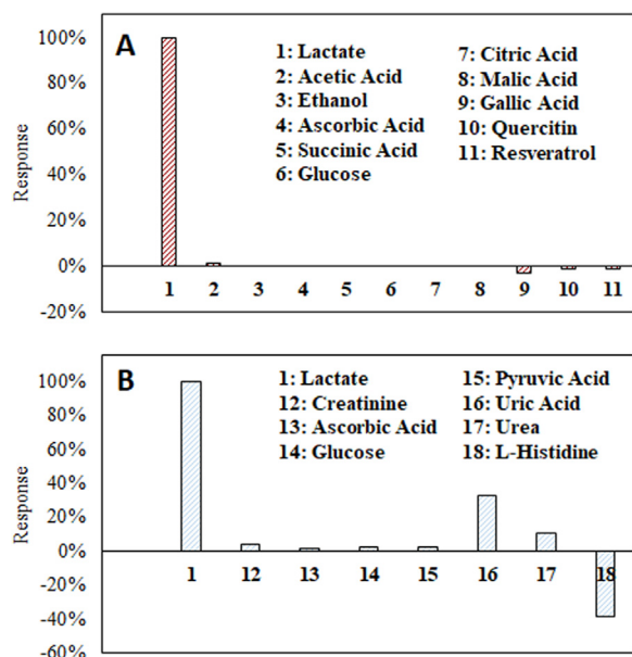
Fig. 2. Percentages of amperometric responses of potential interferents against lactate response, at LO x -Cu-MOF/CS/Pt/SPCE. Eap: 0.15 V (vs SPE Ag/AgCl). (A): wine interferents. Spiked additions of 2 mg L -1 of each interferent compound against lactate: 0.5 mM, in phosphate buffer (0.1 M, pH 7.0); (B): physiological interferents. Spiked additions of components at physiological levels, against 4 mM of lactate, in phosphate buffer saline (0.1 M, pH 7.0; with NaCl (23 mM)).
