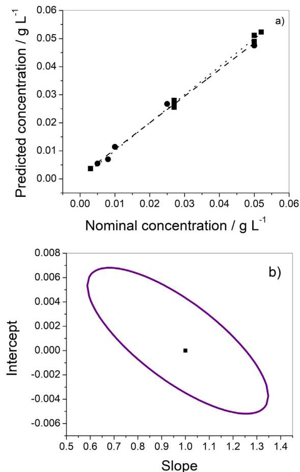
Fig. 6. a) Regression of predicted concentrations vs. nominal values based on weighted least squares (WLS) method corresponding to calibration and validation sets, where: ■ calibration values, • validation values, - - fitting of points of the calibration curve and — fitting of points of the validation values b) EJCR (at a 95% confidence level) of the results obtained for TGs by PLS-1 for the validation set.
