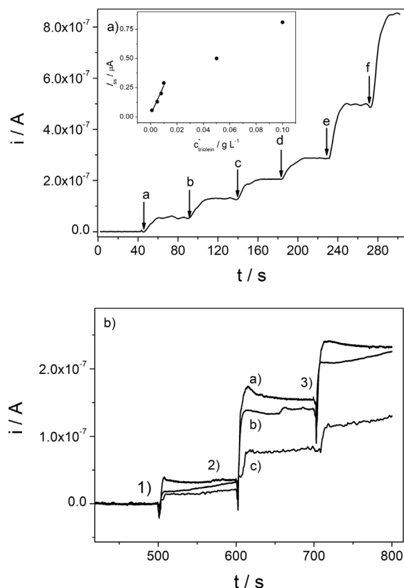
Fig. 3. a) Amperometric measurements performed in pH 8 PBS for different triolein concentration. c_{\text{triolein}}^* : a) 1 \times 10^{-3} , b) 5 \times 10^{-3} , c) 8 \times 10^{-3} , d) 1 \times 10^{-2} , e) 5 \times 10^{-2} and f) 1 \times 10^{-1} g L ^{-1} . Inset: calibration curve. The parameters of linear regression are: slope = (25 \pm 3) \mu\text{A g}^{-1} L, intercept = (1.9 \pm 0.2) \times 10^{-2} \mu\text{A} , r = 0.9709 . b) Amperometric measurements performed for different dilutions of CNP-L: a) 1:100, b) 1:1000 and c) 1:20 for aggregates of triolein of 1) 1 \times 10^{-3} , 2) 5 \times 10^{-3} and c) 8 \times 10^{-3} g L ^{-1} , in pH 8 PBS. E_{\text{app}} = 0.8 V. Stirring speed: 350 rpm.
