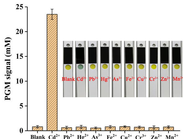
Fig. 3. Selectivity investigation of the PGM-based sensor for \text{Cd}^{2+} and other interfering ions. \text{Cd}^{2+} : 50 nM; other interfering ions: 100 nM. The corresponding error bars represent the standard deviation of three independent measurements.
