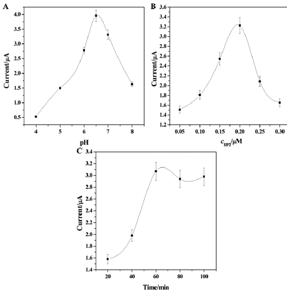
Fig. 4. Effects of (A) pH of detection solution, (B) HP2 concentration, and (C) incubation time of PtPdNPs-HP3 on CV response to 100 pg mL -1 MUC1. Error bars represent standard deviations for three independent experiments.
