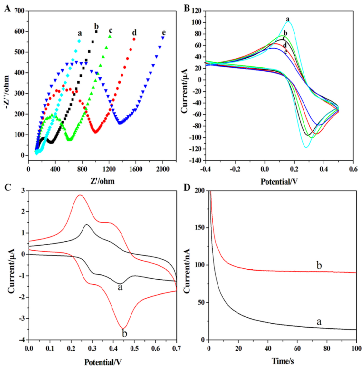
Fig. 3. (A) and (B) are EIS and CVs response of bare gold electrode (a), HP2/Au (b), MCH/HP2/Au (c), MUC1-A/MCH/HP2/Au (d), PtPdNPs-HP3/MUC1-A/MCH/HP2/Au (e) in 5 mM [\text{Fe}(\text{CN})_6]^{3-/4-} solution. (C) and (D) are the CVs and I-t curves of the proposed aptasensor in the absence (a) and presence (b) of 100 \text{pg mL}^{-1} MUC1 in 0.1 M PBS (pH 6.5) containing 0.6 mM TMB and 1.0 mM \text{H}_2\text{O}_2 . Scanrate: 100 \text{mV s}^{-1} ; Potential: +450 mV.
