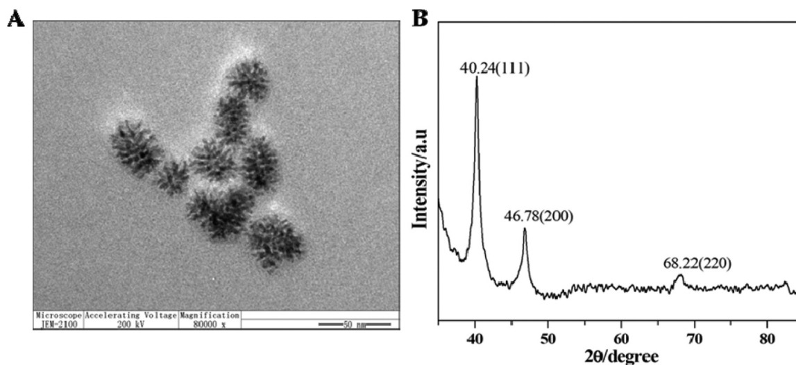
Fig. 1. The TEM image (A) and XRD pattern (B) of PtPdNPs.
