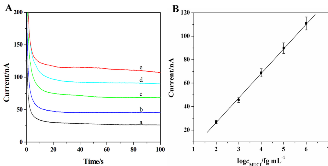
Fig. 5. (A) Chronoamperometric detection of MUC1 at different concentrations at +450 mV. (B) plot of current at 100 s vs logarithmic of MUC1 concentration. Error bars show the standard deviations for three independent experiments.
