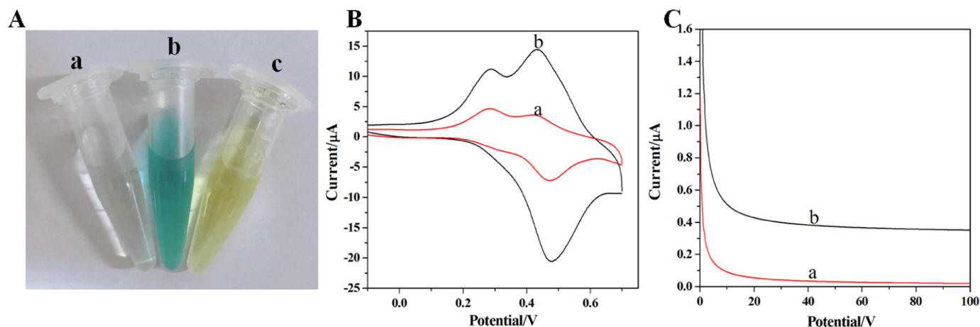
Fig. 2. (A) Photograph of (a) the mixtures of TMB and \text{H}_2\text{O}_2 , (b, c) the mixtures of TMB, \text{H}_2\text{O}_2 , and PtPdNPs before (b) and after (c) adding \text{H}_2\text{SO}_4 . (B) CVs and (C) I - t curves of bare gold electrode (a) and PtPdNPs modified gold electrode (b) in 0.1 M PBS (pH 6.5) containing 0.6 mM TMB and 1.0 mM \text{H}_2\text{O}_2 .
