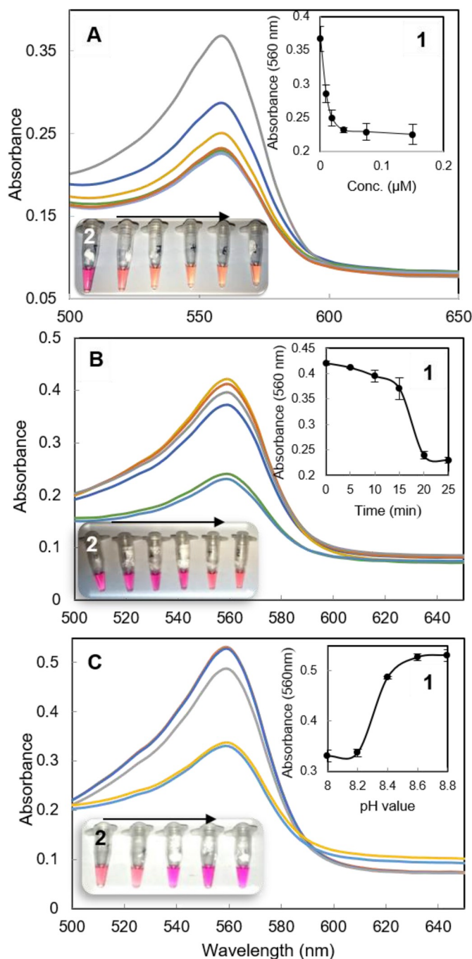
Fig. 3. Optimization of analytical parameters for colorimetric assay. (A) Optimization of PLP concentration was performed at a constant concentration of H_5N_1 target (0.25 \mu M) and different amounts of PLP (from top to bottom: 0, 0.009, 0.018, 0.037, 0.075, 0.150 \mu M). (B) HRCA amplification time optimization was carried out at the optimized concentration of 0.075 \mu M of PLP and 0.25 \mu M of target and different amplification times of 0, 5, 10, 15, 20, 25 min (from top to bottom). (C) pH of amplification buffer optimization was adjusted at a constant concentration of target (0.25 \mu M) and optimized concentration of PLP (75 nM), amplification time of 20 min and in the presence of different pH of amplification reaction 8.8, 8.6, 8.4, 8.2 to 8.0 (from top to bottom). Insets 1 and 2 in graphs A, B, C illustrate the absorbance of samples at 560 nm and a picture of the tubes, respectively (arrows indicate the direction of increasing PLP concentration, amplification time and pH of amplification buffer).
