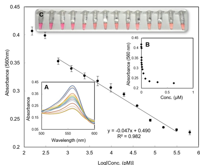
Fig. 4. Calibration curve of H_5N_1 . (A) Determination of absorbance intensity for phenol red at different concentration of targets, from top to bottom, 0, 0.15, 0.30, 0.61, 1.22, 2.44, 4.88, 9.76, 19.53, 39.06, 78.12, 156.25, 312.5 and 625 nM. (B) Standard curve for determination of H_5N_1 target in colorimetric assay. (C) Changes in colors of samples by increasing the concentration of target (from left to right). The main graph represents the data in B on a logarithmic scale. (For interpretation of the references to color in this figure legend, the reader is referred to the Web version of this article.)
