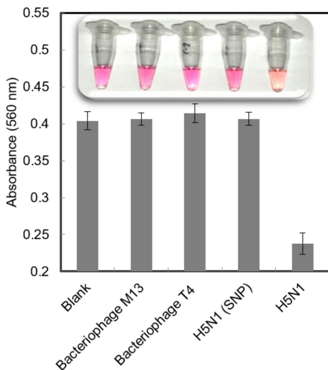
Fig. 5. Selectivity of the assay in the presence of different DNA samples. Selectivity of the system has been evaluated in the presence of different DNA molecules for the PLP targeting H 5 N 1 . These DNA molecules are the bacteriophage M13 and T4 genome, as well as a mutated H 5 N 1 target with a SNP at the ligation site, blank control had no DNA except for PLP and HRCA oligonucleotides. Image shows changes in the colour of the sample with specific target, however the colour for the un-specific targets remains unchanged (tubes are in the same order as the histogram). (For interpretation of the references to color in this figure legend, the reader is referred to the Web version of this article.)
