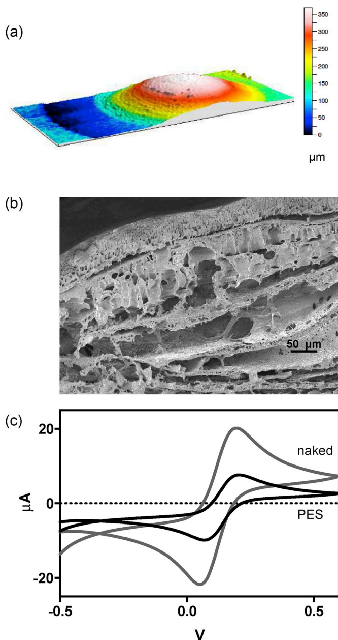
Fig. 1. a) Optical profilometry results of the observations carried out on polyethersulfone-coated screen-printed electrode obtained. Maximum thickness at the center of the electrode is around 300 \mu\text{m} . b) Scanning electron microscopy cross-section of the PES membrane deposited on top of the electrode. c) Cyclic voltammograms of equimolar mixtures ferricyanide/ferrocyanide (1 mM) with and without polyethersulfone membrane.
