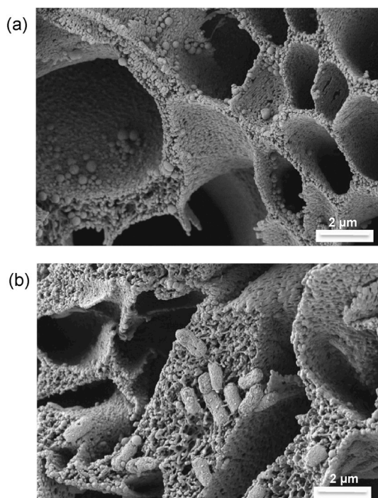
Fig. 3. a) Cross-section image of a PES membrane obtained by Scanning Electron Microscopy. b) Image of a cross-sectioned PES membrane with microorganisms entrapped during phase separation.
