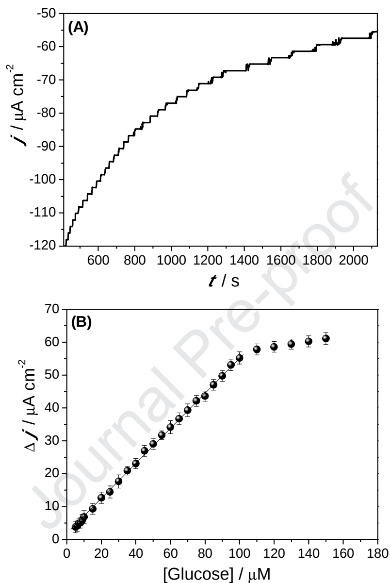
Fig 5 (A) Amperometric response of GOx/PBG ethaline 150/MWCNT/GCE biosensor to glucose in 0.1 M PB solution, pH 7.0; applied potential -0.4 V vs. Ag/AgCl. (B) Calibration curve obtained from injection of increasing concentrations of glucose (0 -150 \mu\text{M} ).
