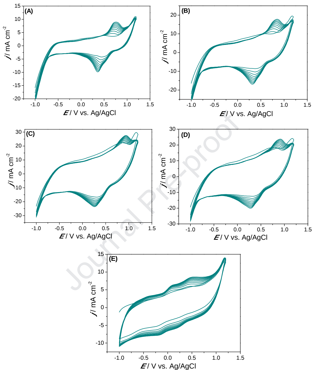
Fig 1. CVs recorded during electropolymerization of BG on MWCNT/GCE in ethaline + (0.5 M \text{H}_2\text{SO}_4 + 10 % \text{H}_2\text{O} ) at scan rates: (A) 50 \text{ mV s}^{-1} ; (B) 100 \text{ mV s}^{-1} ; (C) 150 \text{ mV s}^{-1} ; (D) 200 \text{ mV s}^{-1} ; (E) electropolymerization of BG in aqueous McIlvaine buffer solution pH 4.0 at 150 \text{ mV s}^{-1} .
