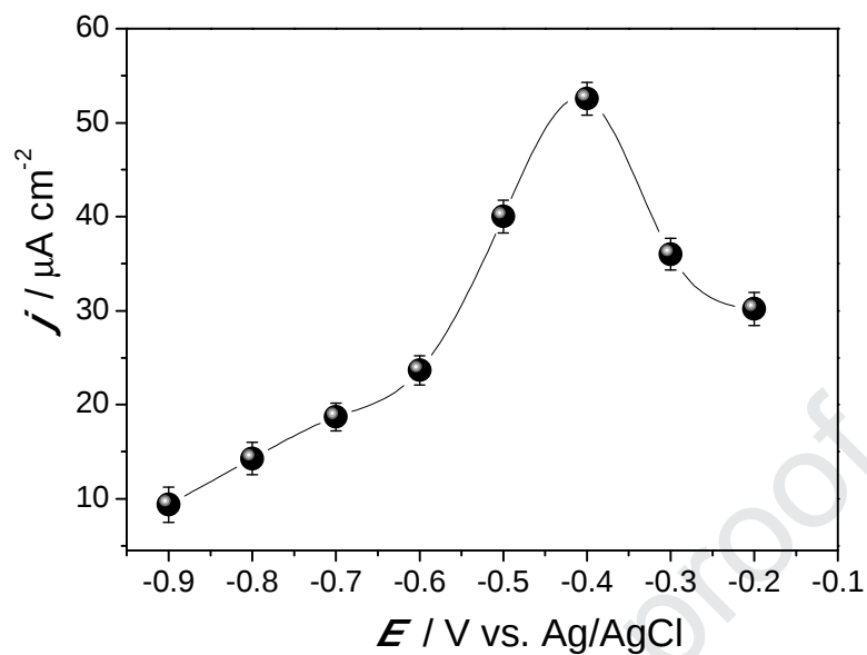
Fig. 4. Dependence of the glucose response at GOx/PBG ethaline 150/MWCNT/GCE on applied potential in 0.1 M PB solution (pH 7.0) in the presence of 100 \mu\text{M} glucose.
