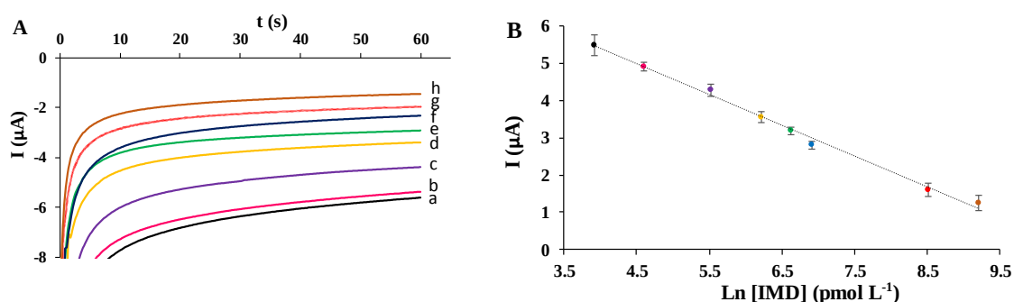
Figure 4. A) Chronoamperograms recorded by applying a potential of -0.2 V for 60 s, after the direct competitive assay performed for increasing concentrations of IMD (a) 50 pmol L -1 , b) 100 pmol L -1 , c) 250 pmol L -1 , d) 500 pmol L -1 , e) 750 pmol L -1 , f) 1000 pmol L -1 , g) 5000 pmol L -1 , h) 10000 pmol L -1 ). (B) Relationship between the analytical signal (current recorded at 60 s) and the logarithm of the IMD concentration.
