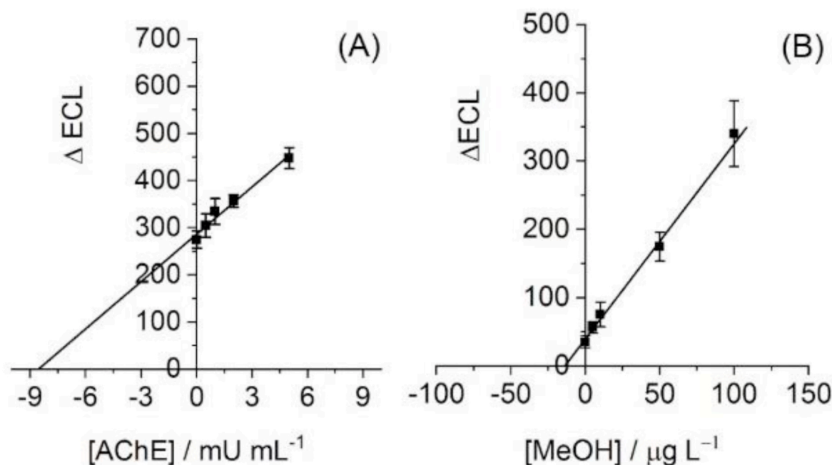
Fig. 5. Quantification of (A) AChE in solutions containing different concentrations of added standard solution of AChE (from 0 to 5 mU mL -1 ), ATCh (0.5 mM) and diluted HS; (B) MeOH in solutions containing different concentrations of added standard (from 0 to 100 \mu g L^{-1} ), AOx (0.05 \mu g mL^{-1} ) and diluted vodka.
