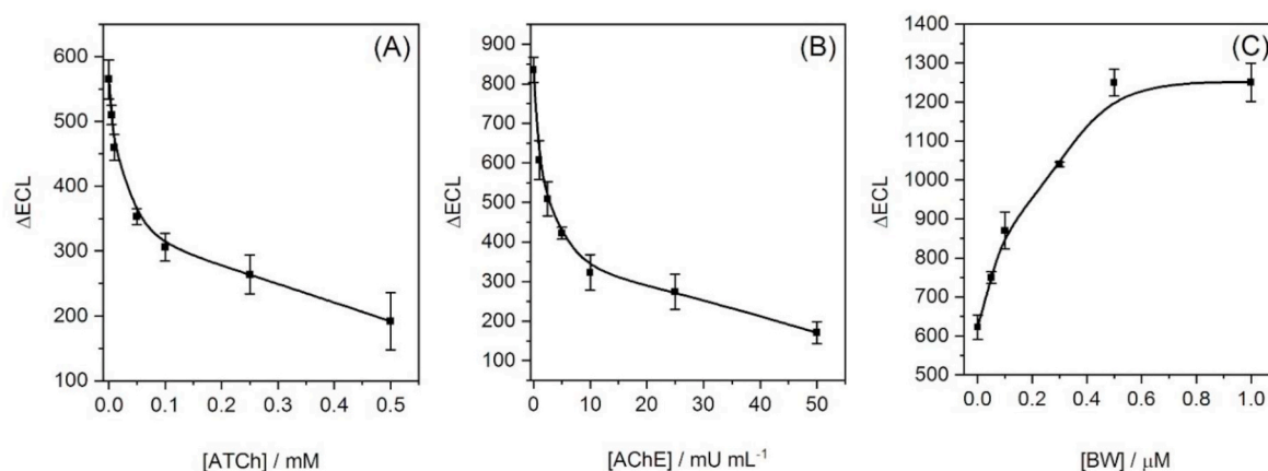
Fig. 3. Calibration curves of (A) ATCh from 0 to 0.5 mM in presence of AChE 50 \text{mU mL}^{-1} , (B) AChE from 0 to 50 \text{mU mL}^{-1} in presence of ATCh 0.5 mM and (C) BW from 0 to 1 \mu\text{M} in presence of AChE 5 \text{mU mL}^{-1} and ATCh 0.5 mM, measured in PBS with \text{H}_2\text{O}_2 10 mM.
