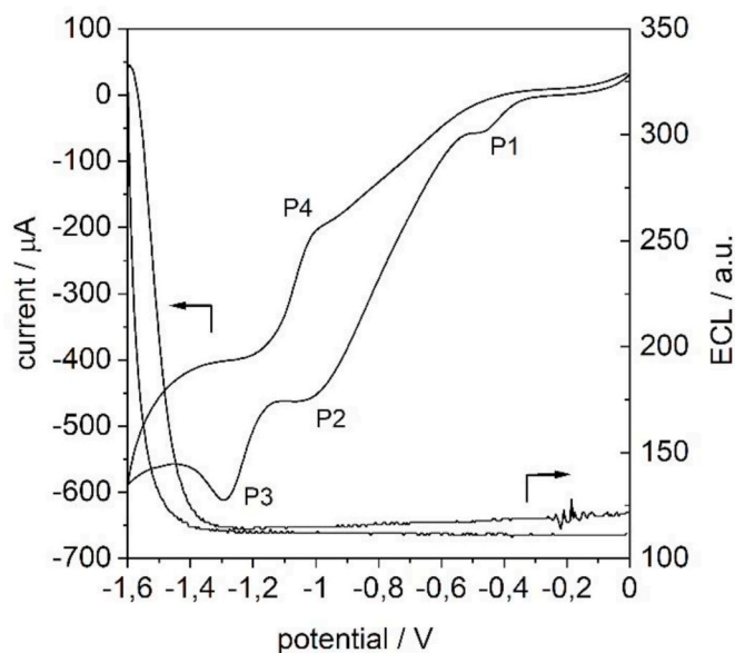
Fig. 2. Cyclic voltammetry and ECL signals from CdS QDs-SPCE in presence of \text{H}_2\text{O}_2 50 mM in PBS.
