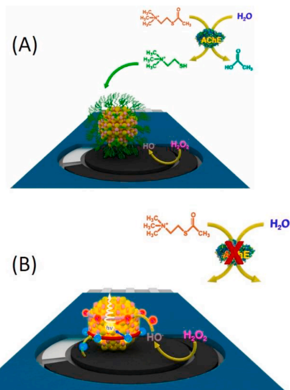
Scheme 1. (A) Enzymatic generation of thiocholine and interaction with the CdS QDs modified electrode. Blocking of the surface and diminution of the ECL signal. (B) Inhibition of AChE through BW inhibitor and increase of the ECL signal.
