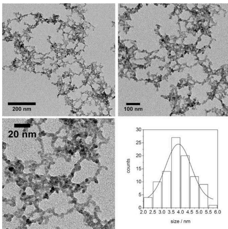
Fig. 1. TEM images from CdS QDs and size histogram.
