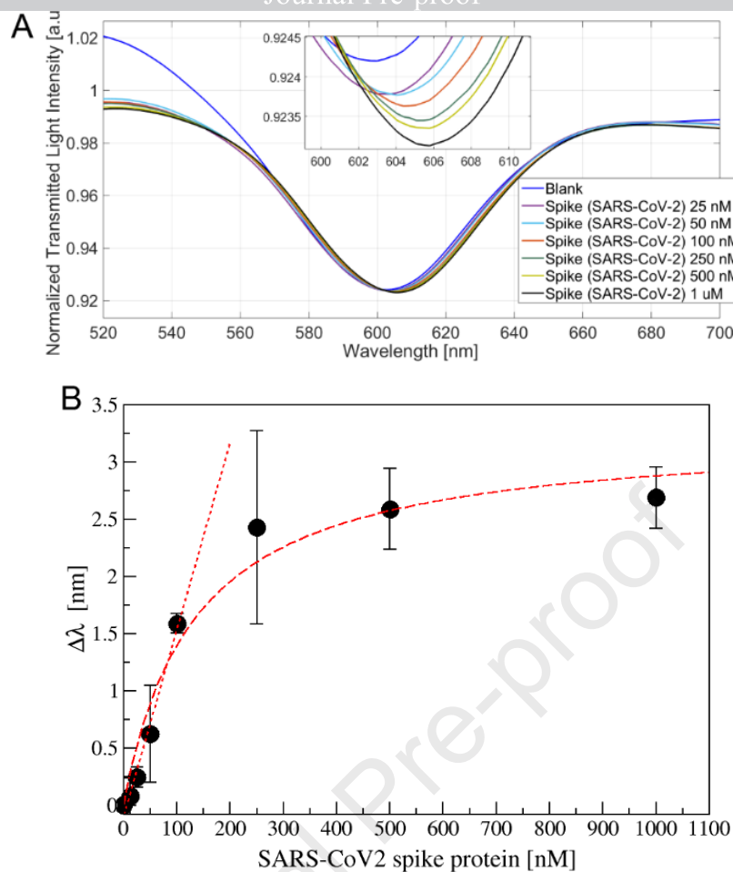
Figure 3. A) Transmission spectra for different SARS-CoV-2 spike protein concentration (25 ÷ 1000 nM) with a zoom of the resonance wavelengths region (inset). B) Resonance shift ( \Delta\lambda ) versus the spike protein concentration (nM), measured on at least three sensor for each value. Data are reported as mean value with standard deviation. Langmuir and linear fitting are also reported.
