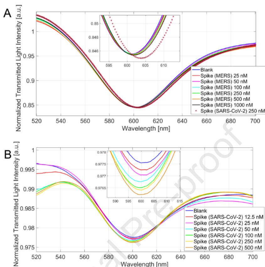
Figure 5. A) Spectra for different MERS spike protein concentrations (25 ÷ 1000 nM) and a SARS-CoV-2 spike protein concentration (250 nM) with a zoom of the resonance wavelengths region (inset). B) Spectra for different SARS-CoV-2 spike protein concentration (12.5 ÷ 500 nM) on the apt-NS-modified platform and a zoom of the resonance wavelengths region (inset).
