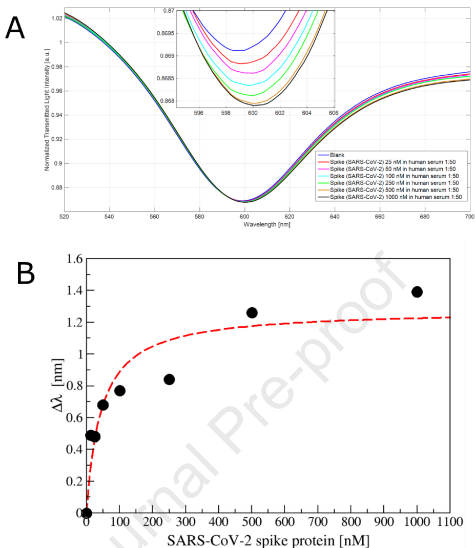
Figure 6. A) SPR transmission spectra, normalized to the spectrum in air, incubating different concentration of SARS-CoV-2 spike protein (25 ÷ 1000 nM) in human serum diluted 1:50 in phosphate buffer on the apt1C- aptamer functionalized POF. Inset: zoom of the resonance wavelengths region. B) Plot of the resonance shift ( \Delta\lambda ), with respect to the blank, versus the spike protein concentration (nM) diluted in human serum (1:50 v/v), reporting also the Langmuir fit.
