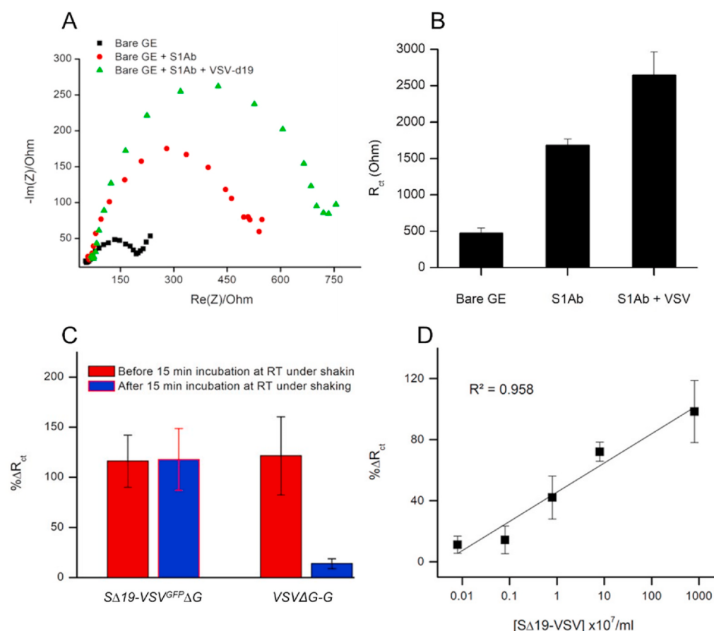
Fig. 4. Detection of SARS-CoV-2 pseudovirus. A) Representative Nyquist plots from measurements of a bare gold electrode (black squares), electrode after functionalization with S1Ab (red circles), and S1Ab-functionalized electrode after incubation in solution containing 2 \times 10^7 /mL SΔ19-VSV GFP ΔG pseudovirus particles (green triangles). B. Corresponding R_{ct} values averaged over 3–5 repetitions. C. Comparison of % \Delta R_{ct} using SΔ19-VSV GFP ΔG vs. VSVΔG-G. Red bars present % \Delta R_{ct} immediately after incubation with either SΔ19-VSV GFP ΔG or VSVΔG-G and blue bars show the same electrodes after 15 min of subtle shaking at room temperature; D) Dependence of % \Delta R_{ct} on SΔ19-VSV GFP ΔG concentration. Data represent the average of three independent experiments (6–8 repetitions each). Error bars represent \pm SD. (For interpretation of the references to color in this figure legend, the reader is referred to the Web version of this article.)
