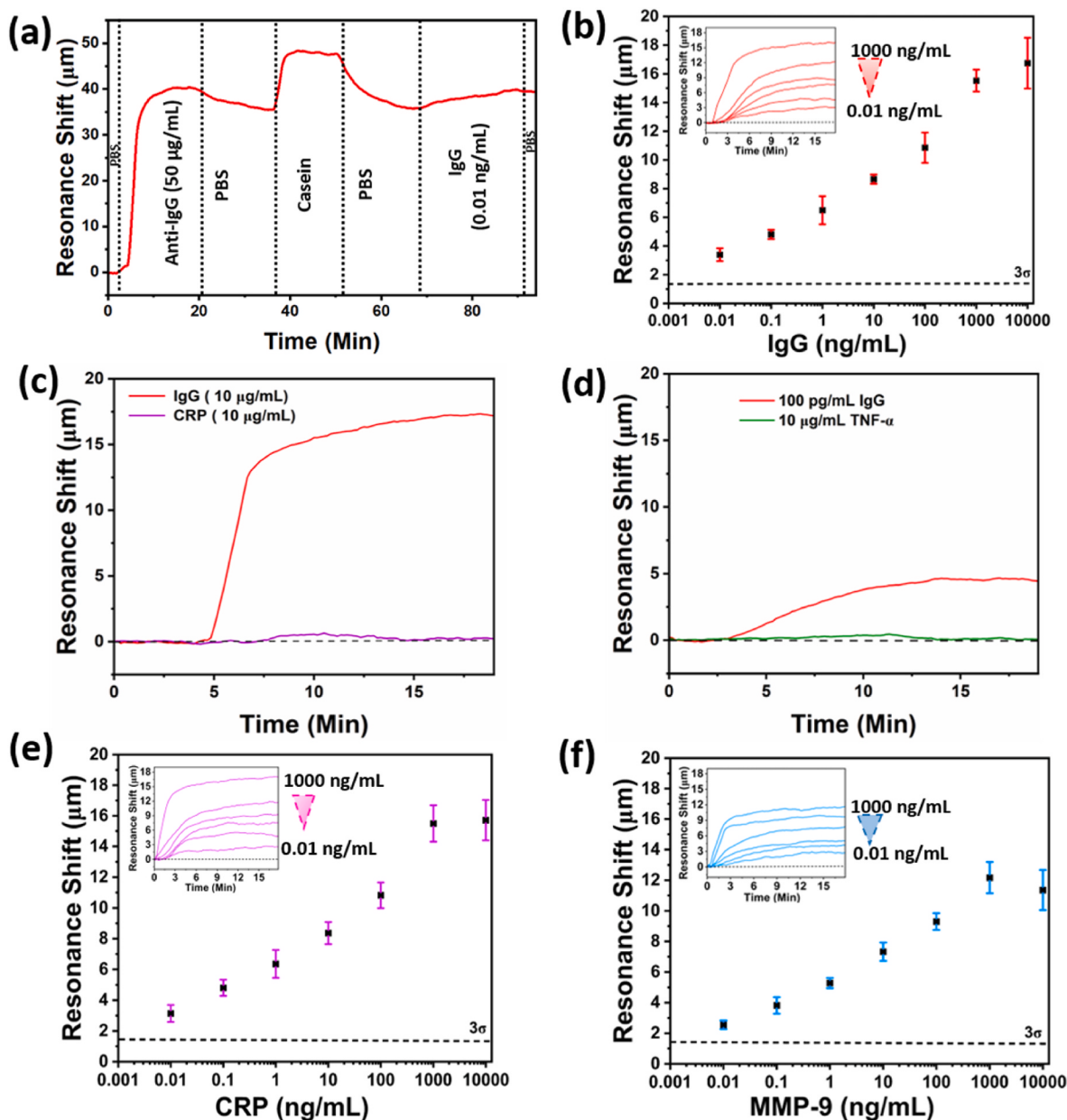
Fig. 4. (a) IgG immunoassay on PDA-functionalised silicon nitride guided mode resonance grating sensors; (b) Resonance shifts observed for an IgG concentration in the range from 0.01 ng/mL to 10,000 ng/mL ( n = 3 \pm \text{SD} ). The inset shows the respective binding curves for an IgG concentration ranging from 0.01 ng/mL to 1000 ng/mL; (c, d) Selectivity test performed on polydopamine coated silicon nitride GMR grating; (c) binding curve for 10 \mu\text{g/mL} of IgG and 10 \mu\text{g/mL} of CRP for a grating functionalised with anti-IgG (50 \mu\text{g/mL} ). For 10 \mu\text{g/mL} IgG, a good shift in the resonance position is observed, while for the same concentration of CRP, only negligible non-specific binding is observed; (d) In the second selectivity test, the sensor was functionalised with anti-IgG (50 \mu\text{g/mL} ), exposed to 100 \mu\text{g/mL} IgG and 10 \mu\text{g/mL} TNF- \alpha . Again, the specific binding is strong while the non-specific binding is negligible; (e and f) Resonance shifts observed for CRP and MMP-9 concentrations in the range from 0.01 ng/mL to 10,000 ng/mL respectively ( n = 3 \pm \text{SD} ). The inset shows the respective binding curves for the protein concentrations ranging from 0.01 ng/mL to 1000 ng/mL.
