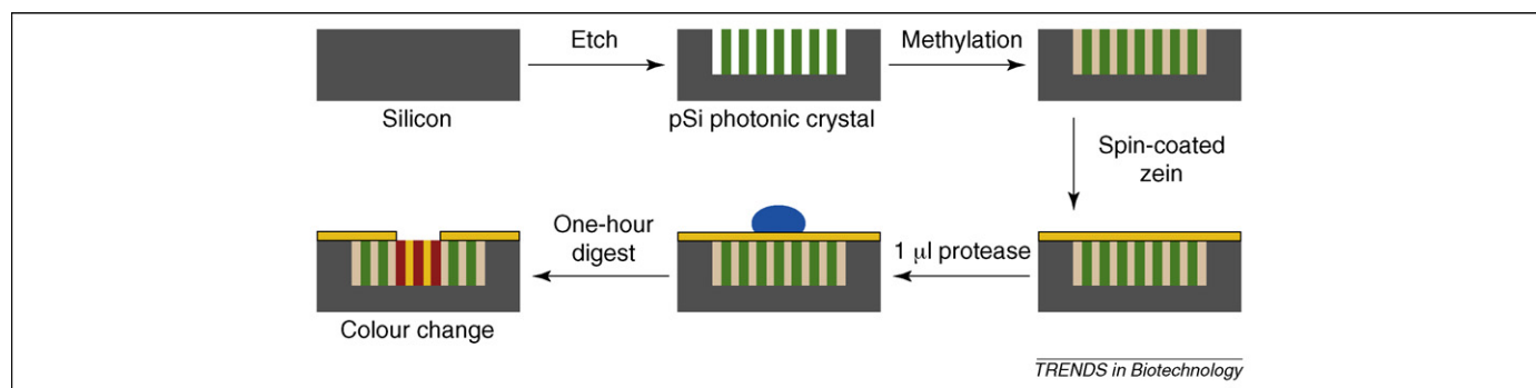
Figure 2. Schematic illustration of an assay for pepsin activity. The pSi sample is first methylated to achieve a hydrophobic interface. It is then spin coated with the protein zein, which is excluded from the porous layer of the photonic crystal. Addition of a protease subsequently results in the digestion of this protein, and proteolytic peptide fragments are able to infiltrate the photonic crystal and lead to a change of refractive index of the porous multilayer, which in turn gives rise to a red shift of the photonic response and a macroscopic colour change. Adapted, with permission, from Ref. [40].
