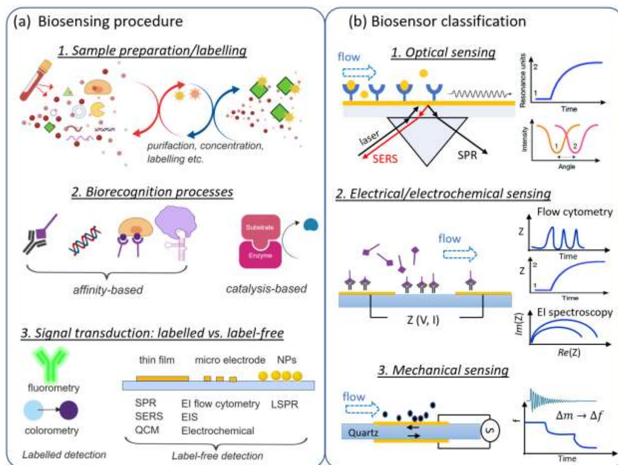
Fig 1. (a) Illustration of biosensing procedure: sample preparation and labeling, which separates, concentrate and label the analytes of interest; biorecognition process associated with antigen-antibody binding, nucleic acid hybridization, specific binding of cell-surface receptor to ligand, aptamer binding to target cells, and catalysis production from enzymic reaction. (b) Classification of biosensors where the biorecognition events are transduced into optical signals such as SERS and SPR, electrical signals such as EI-based flow cytometry, analyte-substrate impedance, and EI spectroscopy, and mechanical signals such as changes in quartz resonance frequency.
