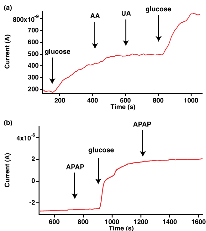
Fig. 6. Current-time response curve of the Au Nc Pt Nf /GOx biosensor to several interfering species in PBS 0.01 M pH 7.4 at +0.15 V (vs. Ag PRE). (a) 0.5 mM glucose, 0.1 M AA, 0.01 M UA and (b) 1 mM glucose, APAP 0.015 M and 0.045 M first and second injection, respectively.
