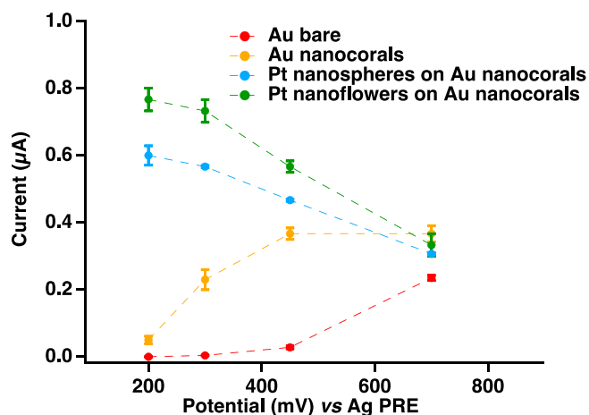
Fig. 2. Effect of applied potential on the amperometric response to 20 \mu\text{M} \text{H}_2\text{O}_2 at (red) bare Au, (orange) Au nanocorals, (green) \text{Au}_{\text{Nc}}\text{Pt}_{\text{Nf}} and (blue) \text{Au}_{\text{Nc}}\text{Pt}_{\text{Nsp}} electrodes. Amperometric measurements were performed at various levels of the applied potential in stirred 0.01 M PBS pH 7.4 solution by injecting 20 \mu\text{M} \text{H}_2\text{O}_2 . (For interpretation of the references to colour in this figure legend, the reader is referred to the web version of this article.)
