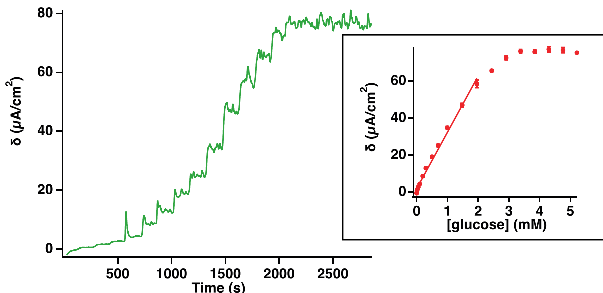
Fig. 5. Amperometric response obtained to successive additions of glucose in a stirred 10 ml solution of PBS 0.01 M pH 7.4 at +0.15 V (vs. Ag PRE) using \text{Au}_{\text{Nc}}\text{Pt}_{\text{Nf}}/\text{GOx} biosensor. The inset shows the amperometric current density response of the biosensor as a function of glucose concentration.
