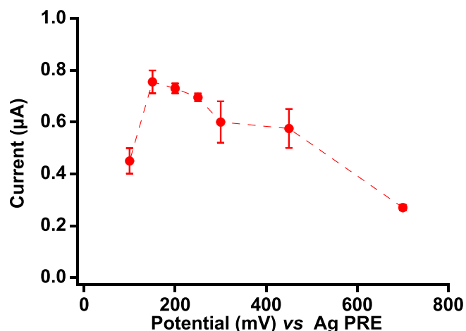
Fig. 4. Effect of applied potential on the amperometric response at \text{Au}_{\text{Nc}}\text{Pt}_{\text{Nf}}/\text{GOx} electrode towards the detection of 1 mM glucose.
