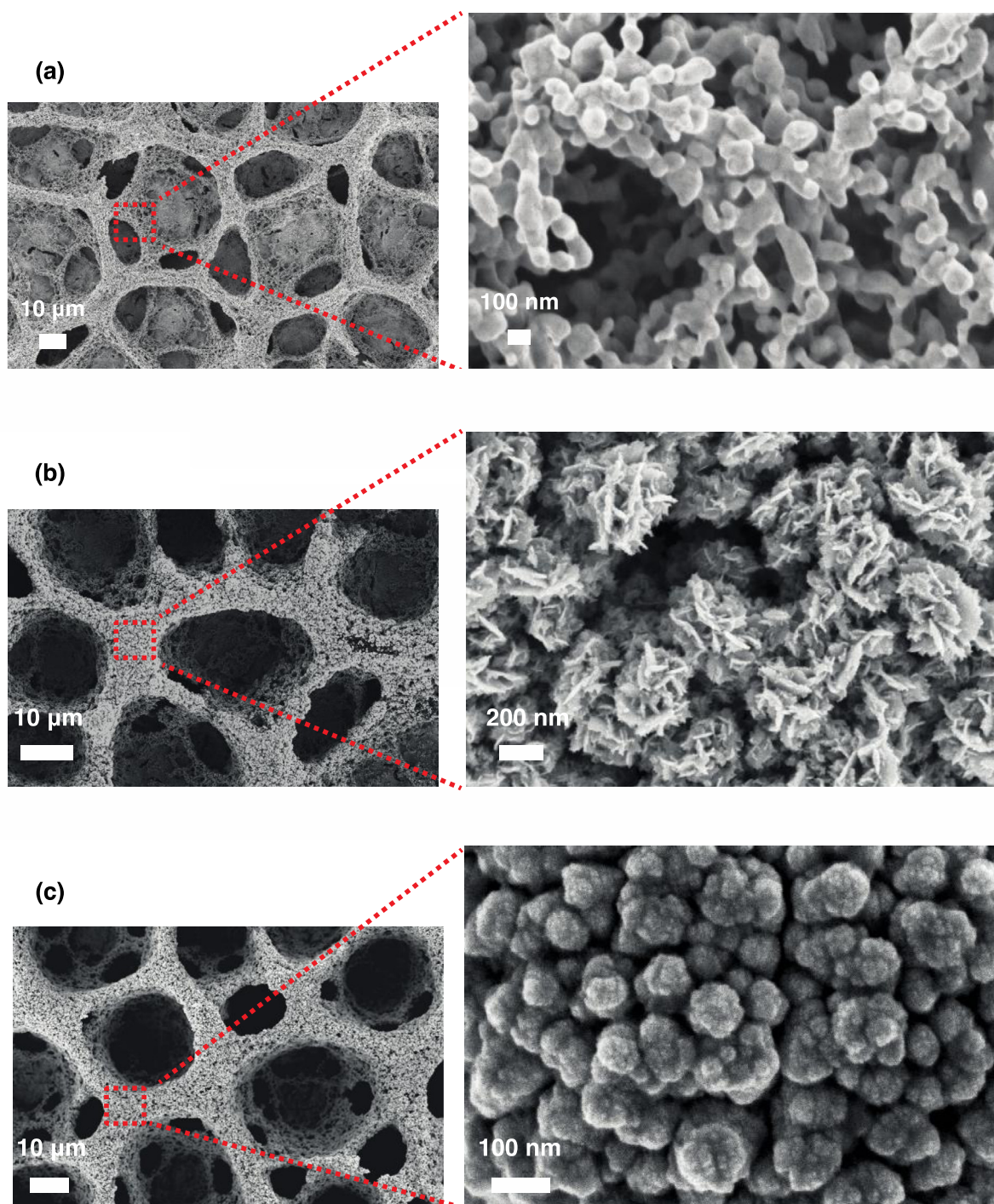
Fig. 1. SEM images of (a) Au nanocorals, (b) Au nanocorals with Pt nanoflowers ( -1 V for 90 s from tetravalent Pt) and (c) with Pt nanospheres ( -0.2 V for 200 s from divalent Pt).
