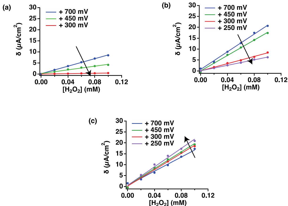
Fig. 3. Effect of the applied potential on the sensitivity by using (a) Au bare, (b) Au nanocorals and (c) \text{Au}_{\text{Nc}}\text{Pt}_{\text{Nf}} .
