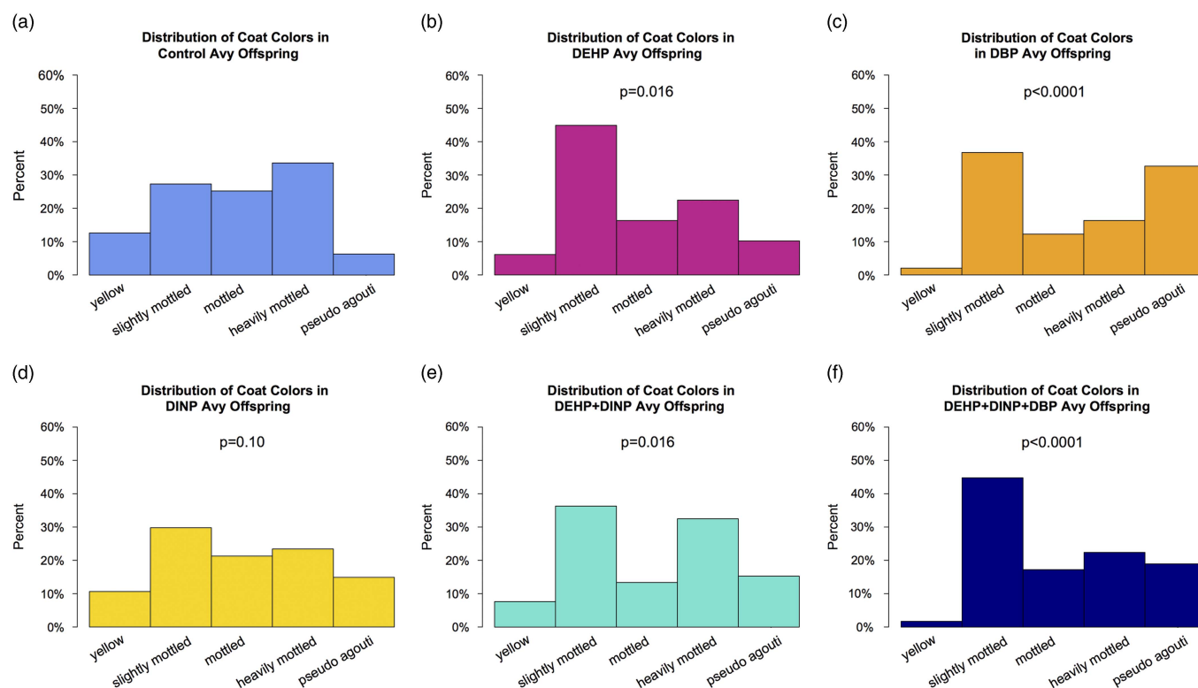
Fig. 4. Coat color distributions of A^{y/a} offspring across exposure groups. Coat color distributions for each exposure group were compared with the control using a \chi^2 goodness-of-fit test. (a) Control coat color distribution; n = 16 litters, 50 animals. (b) Diethylhexyl phthalate (DEHP) coat color distribution; P = 0.016 ; n = 14 litters, 49 animals. (c) Dibutyl phthalate (DBP) coat color distribution; P < 0.0001 ; n = 14 litters, 49 animals. (d) Diisononyl phthalate (DINP) coat color distribution; P = 0.10 ; n = 15 litters, 47 animals. (e) DEHP + DINP coat color distribution; P = 0.016 ; n = 16 litters, 55 animals. (f) DEHP + DBP + DINP coat color distribution; P < 0.0001 ; n = 17 litters, 61 animals. A^{y/} , viable yellow agouti.
