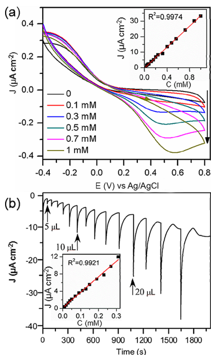
Figure 3. (a) Cyclic voltammetry of the \text{Fe}_{30}\text{Pt}_{70} NP electrode (with a scan rate of 50 \text{ mV s}^{-1} ) in the absence and presence of different ascorbic acid (AA) concentrations in a 10 mM PBS solution. (b) Corresponding amperometric response to successive addition of five aliquots of 5, 10, and 20 \mu\text{L} of a stock solution of 50 mM AA to a 10 mM PBS solution. The linear relationships between the peak current density at 0.5 V and the concentration over different concentration ranges are shown in the respective insets.
