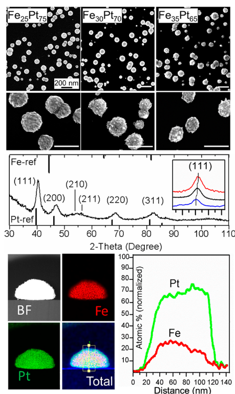
Figure 1. Top panel: SEM images of FePt alloy NPs with three different compositions, Fe 25 Pt 75 , Fe 30 Pt 70 , and Fe 35 Pt 65 , obtained from amperometry at -1.1 V vs Ag/AgCl for 60 s deposition (scale bars show 200 nm). Middle panel: Comparison of the GIXRD pattern of Fe 25 Pt 75 alloy NPs with the reference patterns for Fe bcc (PDF2 01-085-1410) and Pt fcc (PDF2 004-0802), with the shift in the (111) peaks for Fe 25 Pt 75 , Fe 30 Pt 70 , and Fe 35 Pt 65 NPs shown in the inset (bottom to top). Bottom panel: Bright-field (BF) STEM image of a typical Fe 25 Pt 75 NP and its corresponding Fe and Pt EDX elemental maps obtained by EDX analysis. The uniform distributions of both Fe and Pt elements in the elemental maps of the NP show mixed alloy NP formation, with a self-organized Pt-enriched region on the surface as indicated by the line scans throughout the NP.
