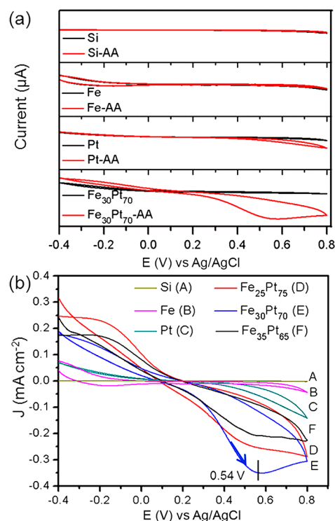
Figure 2. (a) Cyclic voltammograms of a bare Si electrode and electrodes electrodeposited with pristine Fe nanoparticles (NPs), pristine Pt NPs, and Fe 30 Pt 70 alloy NPs, all in a 10 mM PBS solution without and with 1 mM ascorbic acid (AA). (b) Cyclic voltammograms of Si electrode, electrodes with Fe NPs, Pt NPs, and Fe 25 Pt 75 , Fe 30 Pt 70 , and Fe 35 Pt 65 alloy NPs in a 10 mM PBS solution with 1 mM ascorbic acid (AA). Scan rate is 50 \text{ mV s}^{-1} .
