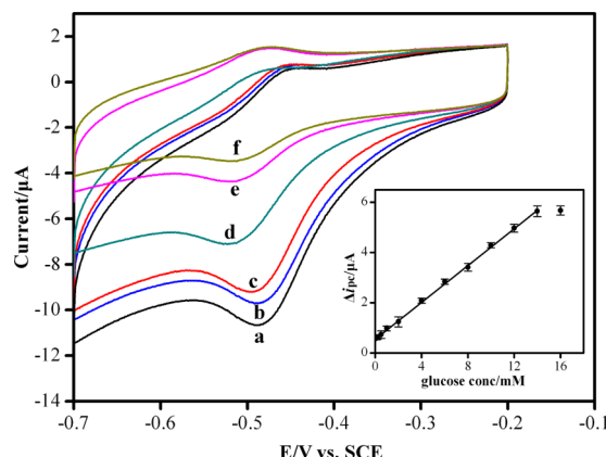
Figure 4. CVs of Nafion/GOx-yeast/MWNTs/GCE in PBS buffer (pH 7.4) containing different concentrations of glucose: 0.0 mM (trace a), 0.1 mM (trace b), 0.5 mM (trace c), 2.0 mM (trace d), 8.0 mM (trace e), and 12.0 mM (trace f). Scan rate = 50 \text{ mV s}^{-1} . Inset shows a typical calibration graph of the glucose biosensor.
