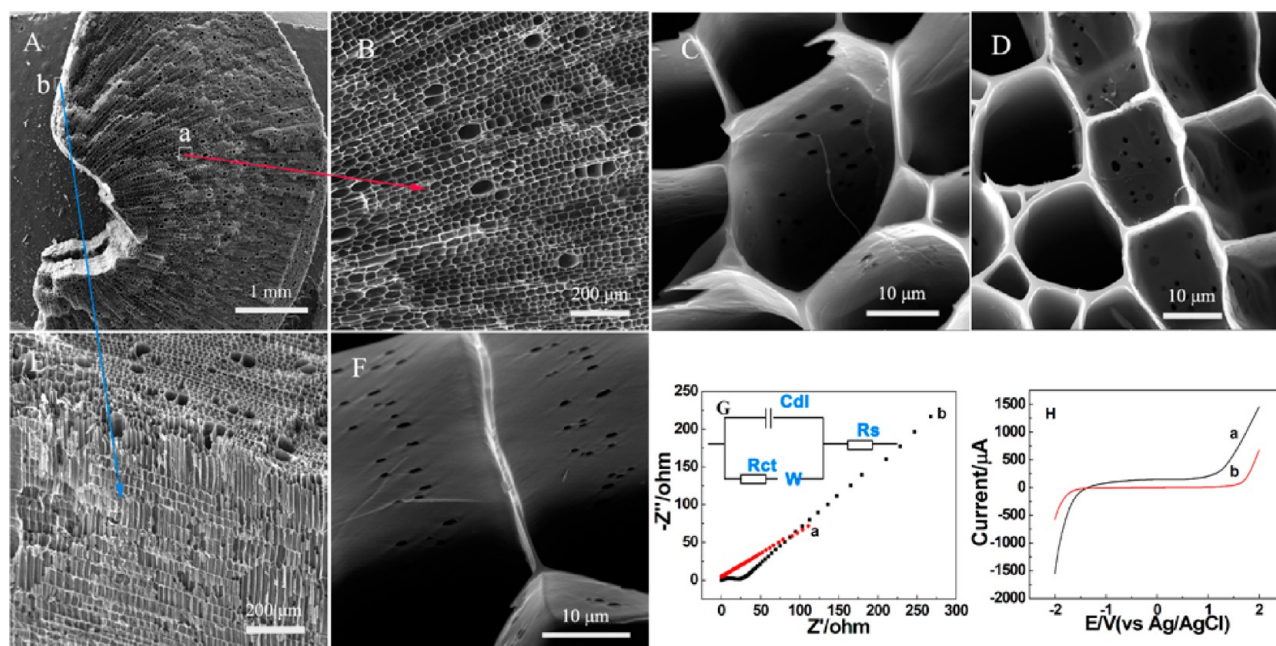
Figure 2. (A–F) SEM images of 3D-KSCs: (A) overview of a piece of cleaved 3D-KSCs, (B) top-view image, (C,D) images magnified from position B, (E) side-view image, (F) image magnified from position E, (G) Nyquist plots at the 3D-KSCs electrode (curve a) and GCE (curve b) in 5 mM \text{Fe}(\text{CN})_6^{3-/4-} containing 0.1 M KCl. The inset is the equivalent circuit. (H) LSVs of the 3D-KSCs electrode (curve a) and GCE (curve b) in 0.1 M PBS (pH 7.0) at 50 \text{ mV s}^{-1} .
