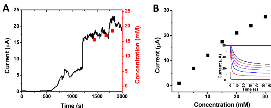
Figure 6. (A) Real-time response of the tattoo biosensor during a cycling exercise (left y-axis) and corresponding lactate concentrations (right y-axis); red dots represent the lactate concentrations in the sweat collected at these times. (B) In vitro calibration curve of tattoo biosensor at 37 °C; inset, amperometric response to different lactate concentrations up to 30 mM with 5 mM increments.
