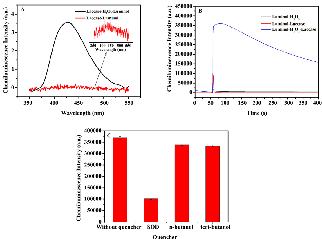
Figure 1. Characterization of the luminol- \text{H}_2\text{O}_2 -laccase CL reaction. (A) CL spectra for the luminol- \text{H}_2\text{O}_2 -laccase and luminol-laccase CL reactions. (B) Kinetic characteristics of the luminol- \text{H}_2\text{O}_2 -laccase, luminol- \text{H}_2\text{O}_2 , and luminol-laccase reactions. (C) Effects of quenchers on the luminol- \text{H}_2\text{O}_2 -laccase CL intensity. Conditions: 0.1 \text{ mg mL}^{-1} SOD, 0.1 \text{ mol L}^{-1} n -butanol, 0.1 \text{ mol L}^{-1} tert -butanol.
