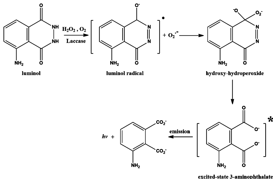
Scheme 2. Mechanism of Laccase Enhanced Luminol–H 2 O 2 Chemiluminescence System
