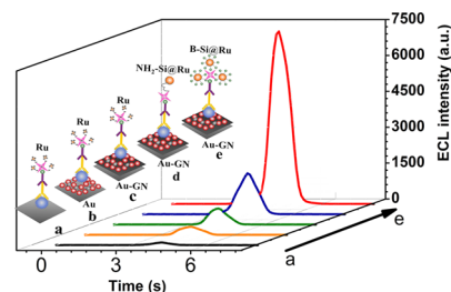
Figure 5. ECL responses of (a) Ru(BPY) 3 /SA/B-Ab 2 /Ab 1 /BSA/Ag/GCE, (b) Ru(BPY) 3 /SA/B-Ab 2 /Ab 1 /BSA/Ag/Au NPs/GCE, (c) Ru(BPY) 3 /SA/B-Ab 2 /Ab 1 /BSA/Ag/Au-GN/GCE, (d) NH 2 -Ru@SNPs/SA/B-Ab 2 /Ab 1 /BSA/Ag/Au-GN/GCE, and (e) B-Ru@SNPs/SA/B-Ab 2 /Ab 1 /BSA/Ag/Au-GN/GCE.
