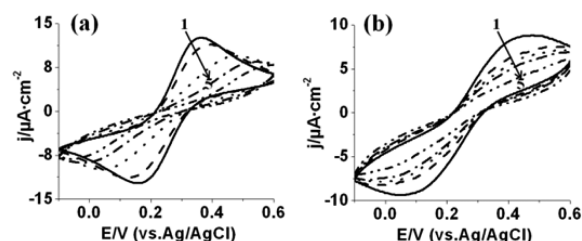
Figure 2. Cyclic voltammogram obtained, first for the TLR5 sensor before ligand immersion, and then after exposure to various concentrations of (a) S. typhimurium , a Gram-negative species, and (b) B. subtilis , Gram-positive. The corresponding concentrations of species are 0 (before immersion), 0.1, 0.5, 1, and 2 \mu\text{M} from 1 to 5. The scan rate was 0.1 \text{ V} \cdot \text{s}^{-1} , and measurements were carried out in a 5 mM/5 mM \text{Fe}(\text{CN})_6^{3-/4-} aqueous solution with 1 M \text{NaClO}_4 as the supporting electrolyte.
