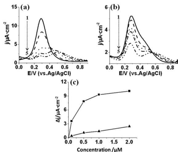
Figure 3. Square-wave voltammogram obtained, first for the TLR5 sensor before ligand immersion, and then after exposure to various concentrations of (a) S. typhimurium , a Gram-negative species, and (b) B. subtilis , Gram-positive. The corresponding concentrations of species are 0 (before immersion), 0.1, 0.5, 1, and 2 \mu\text{M} from 1 to 5. A plot (c) summarizing the current density change ( \Delta j ) upon exposure of the TLR5 sensor platform to various concentration of the respective ligands, S. typhimurium (■) and B. subtilis (▲).
