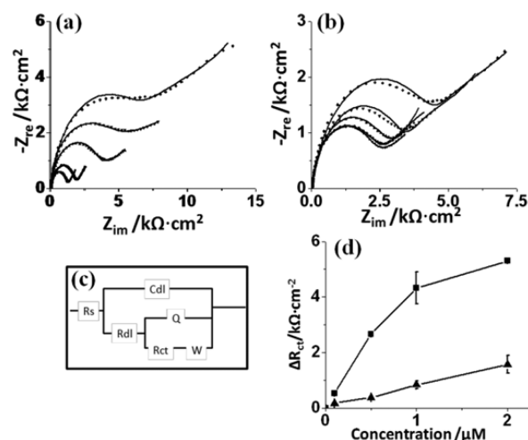
Figure 4. Nyquist plots before and after exposing the TLR5 sensor to ligands of S. typhimurium (a) and B. subtilis (b) at solution concentrations of 0.1, 0.5, 1, and 2 \mu\text{M} , respectively. Impedance results were recorded from 100 kHz to 0.1 Hz. The continuous lines fitted through the scatter plots are impedance curves calculated using the circuit model shown in panel c for estimation of the film Rct. Within the circuit model, R_s is the solution resistance, R_{dl} is the double layer resistance, R_{ct} is the film resistance, C_{dl} is the double layer capacitance, Q is the constant phase element of the film, and W is the finite length Warburg impedance. The values for each element resulting from the modeling process are included in the Supporting Information Tables S1 and S2. (d) Plots of \Delta R_{ct} before and after exposing the TLR5 sensor to varying concentrations of S. typhimurium (■) and B. subtilis (▲) ligands, respectively. \Delta R_{ct} = R_{ct} (after immersion at a concentration) – R_{ct} (before immersion). The EIS measurements were carried out in an electrochemical cell containing a 5 mM/5 mM \text{Fe}(\text{CN})_6^{3-/4-} aqueous solution with 1 M \text{NaClO}_4 as the supporting electrolyte.
